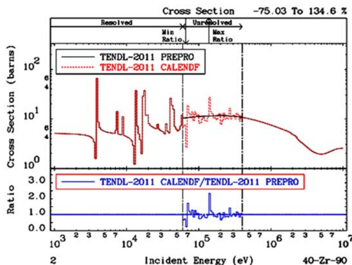
Figure 5: CALENDF improves the cross-section description in the URR energy range
