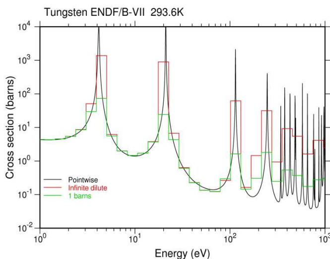
Figure 5: CALENDF improves the cross-section description in the URR energy range
