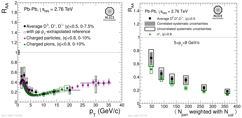
Fig. 4. Comparison of the average D^0, D^+, D^{*+} R_{AA} to the charged pion R_{AA} as a function of the transverse momentum in the most central collisions (0–7.5%) (left) and as a function of the collision centrality for 5 < p_T < 8 GeV/ c (right).
