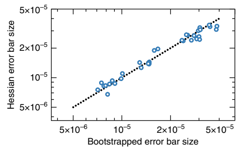
Figure 8 | Comparison of error bar generation techniques. When computing error bars on GST estimates in this manuscript, we typically use LR confidence regions, computed using the Hessian of the log-likelihood function. However, another common approach is through parametric bootstrapping. Here we show a log-log scatter plot of error bars on gate elements from GST estimate of our data from 30 March 2015. The x axis corresponds to error bars calculated via parametric bootstrapping, whereas the y axis corresponds to likelihood ratio (LR) confidence regions computed using the Hessian of the log-likelihood function. The dotted line corresponds to y = x . Both methods are described in the methods section ‘Error Bars’. The strong correlation shown here demonstrates the consistency between parametric bootstrapping techniques and LR confidence regions.
