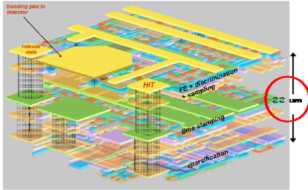
Figure 8 – 3D circuit diagram and 3D layout of pixel cell
