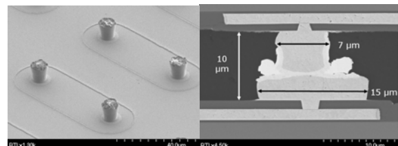
Figure 1: (l) 7 micron diameter pillars on 20 micron pitch, (r) cross section of solder connection showing height of connection.
