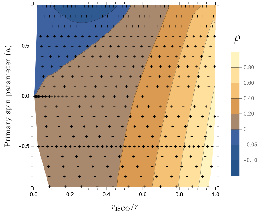
Figure 12. The linear in mass ratio correction, \rho , to the periaapsis advance, W , as a function of distance from the ISCO r_{\text{ISCO}}/r and the spin of the primary, a . The contours show that \rho grows larger as the radius of the inspiral approaches the ISCO. \rho is positive for most of the parameter space, including for all retrograde orbits, implying that in these regions the self-force acts against the geodesic periaapsis advance. However, for all prograde orbits, there is a region (in blue) where this correction is negative meaning the self-force instead increases the rate of periaapsis advance. The region where this occurs grows larger as a increases. The black crosses mark the location of the underlying data from reference [88] used to calculate the contour plot.
