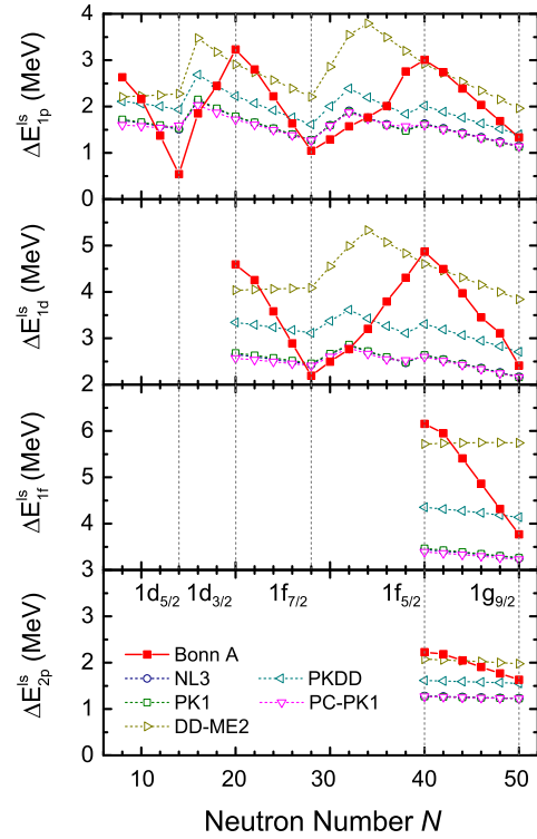
Fig. 2. (Color online) From top to bottom panel, 1p, 1d, 1f, and 2p spin-orbit splittings of N -neutron drops in a HO trap ( \hbar\omega = 10 MeV) calculated by the RBHF theory using the Bonn A interaction, in comparison with the results obtained by various RMF density functionals.
