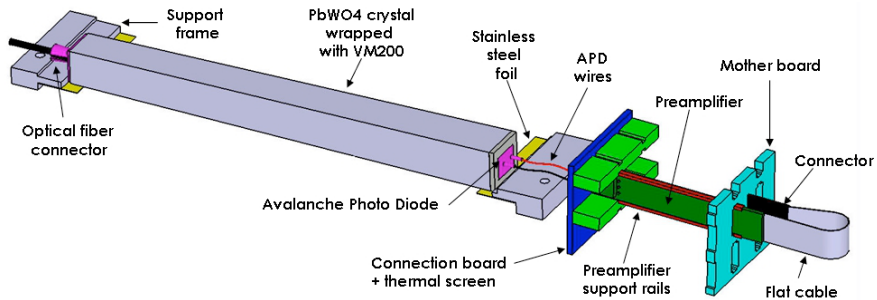
Figure 4.12: Rendered view of an HPS Ecal module consisting of a 16 cm PbW 4 crystal, Avalanche Photodiode and preamplifier board.
