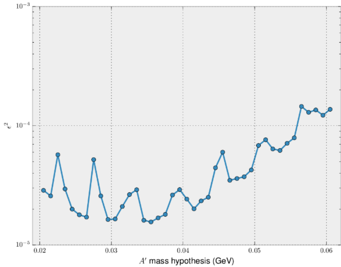
Figure 7.9: Upper limits on the coupling strength.
