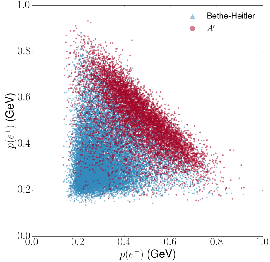
Figure 3.4: Scatter plot of the positron momentum versus the electron momentum of pairs from Bethe-Heitler background (blue) and 50 MeV A' signal events (red). The kinematics of the irreducible radiative background are indistinguishable from A' signal events within an invariant mass window, \delta m , centered at m_{A'} and can be used to analyze the rate of A' signal production.
