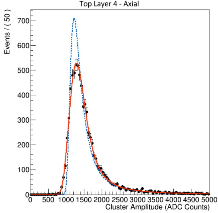
Figure 5.8: Distribution of cluster charge exhibiting the characteristic Landau shape. The cluster charge was fit with a Landau (dashed blue line) convoluted with a Gaussian (convolution shown in red) in order to extract the most probable value.
