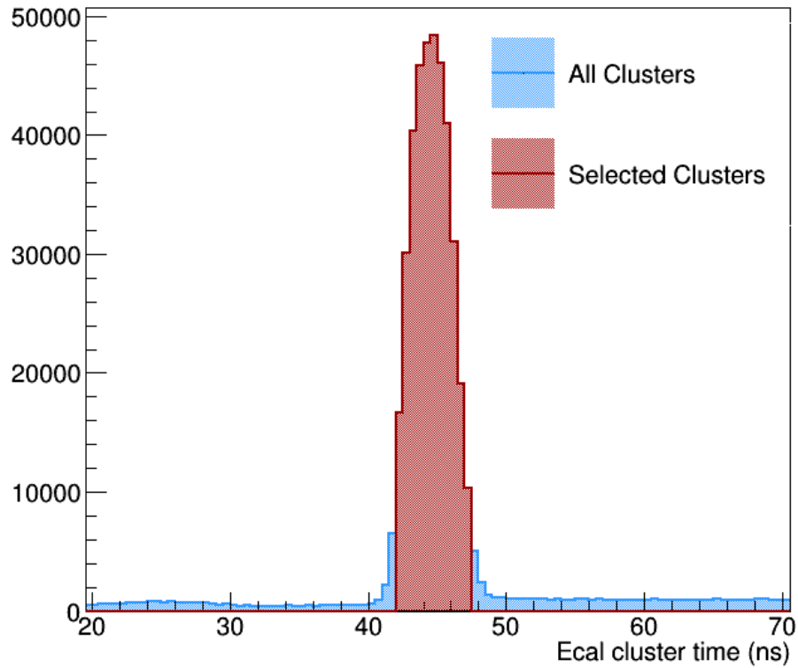
Figure 6.2: Cluster time of all Ecal clusters in an event (blue). The time of cluster is required to be between 42 ns and 47.5 ns (red) in order to ensure that it falls within the trigger window.
