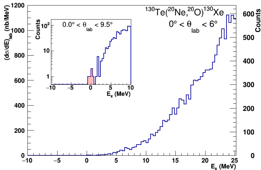
Figure 5. Excitation energy spectrum for the ^{130}\text{Te}(^{20}\text{Ne}, ^{20}\text{O})^{130}\text{Xe} DCE reaction at 306 MeV incident energy and 0.0^\circ \leq \theta_{lab} \leq 6.0^\circ angular range. A zoomed view for E_x < 10 MeV and full angular range 0.0^\circ \leq \theta_{lab} \leq 9.5^\circ is shown in the inset. The ^{130}\text{Te}_{g.s.} \rightarrow ^{130}\text{Xe}_{g.s.} region ( -1 \text{ MeV} \leq E_x \leq 1 \text{ MeV} ) is indicated with the red hatched area. Figure from Ref. [21].
