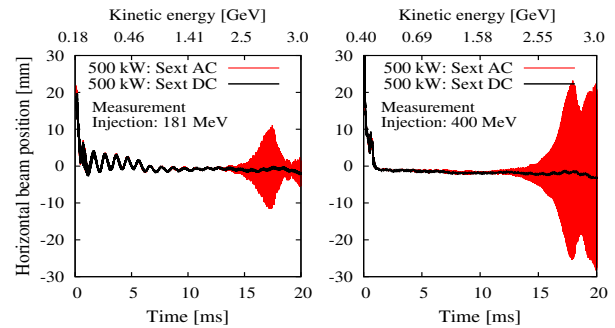
Figure 3: Measurement results of beam instability for 500 kW equivalent beam. The instability occurs only when AC chromatic correction is done. The 400 MeV injected beam (right) is more unstable than that the 181 MeV one (left).
