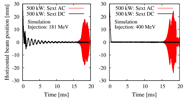
Figure 4: Simulation results for the corresponding measurements as shown in Fig. 3.
