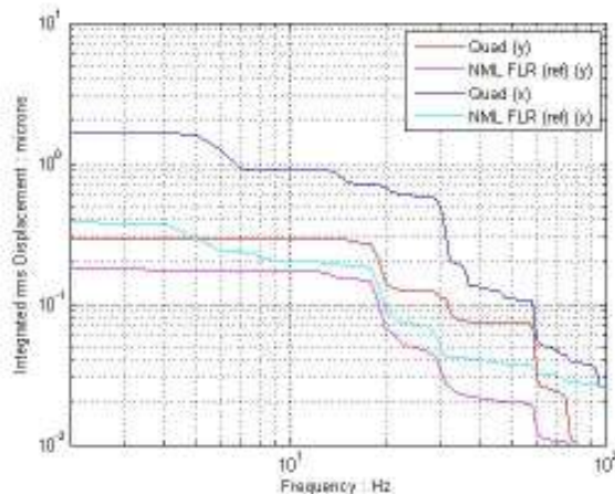
Figure 3: Integrated displacement baseline for NML.
