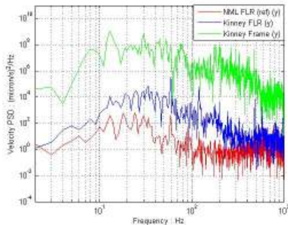
Figure 7: NML vertical PSD velocity Kinney test.
