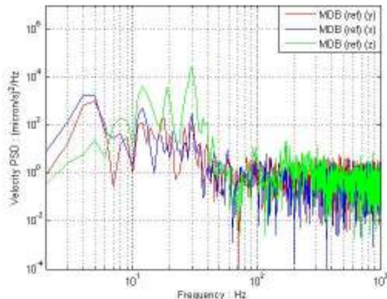
Figure 6: Velocity PSD baseline for MDB.
