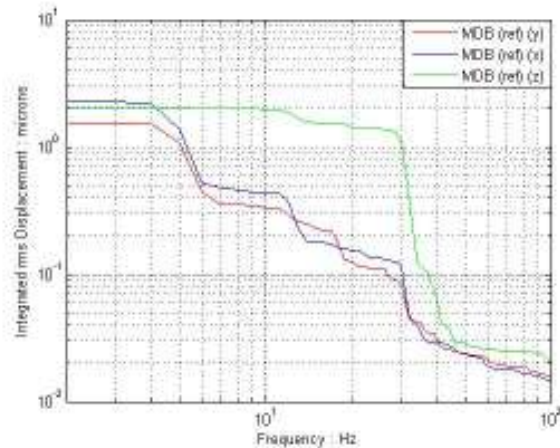
Figure 5: Integrated displacement baseline for MDB.
