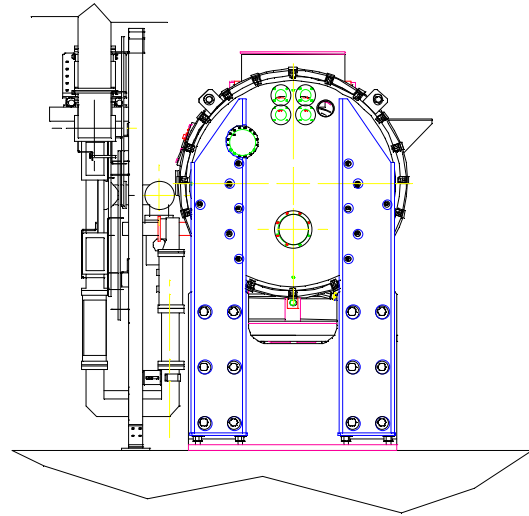
Figure 1: Upstream end view of CM1.
