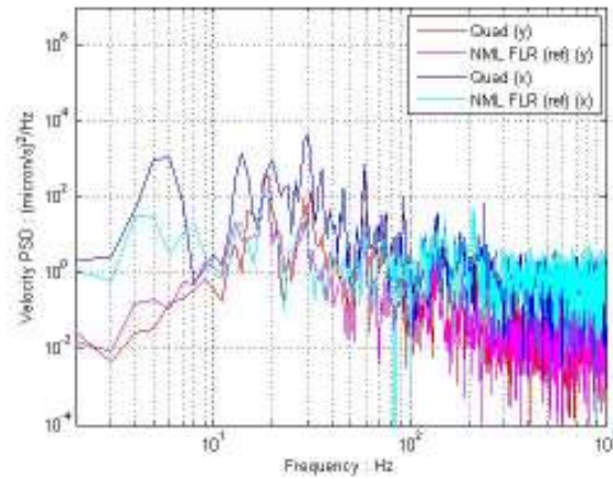
Figure 4: Velocity PSD baseline for NML.
