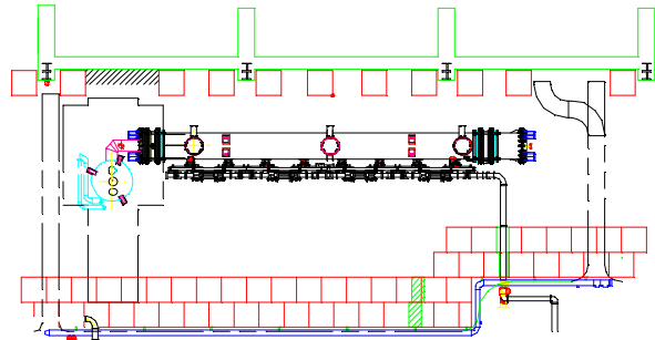
Figure 2: Plan view of CM1 at NML.
