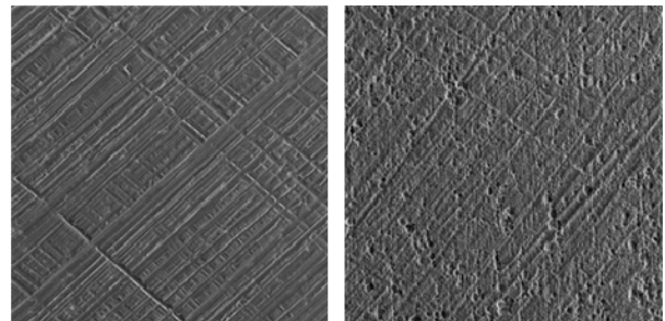
Figure 2: Image of honed surface finish before and after the etching process.
