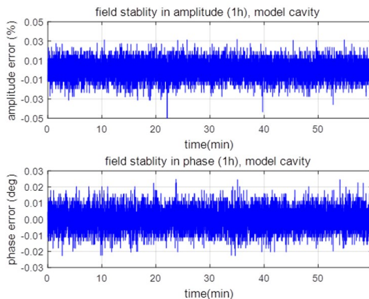
Figure 6: Amplitude and phase error measured on a warm cavity with \text{ref\_amp}=0.8 . Errors are referring to differences between feedback and reference signals.
