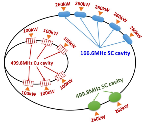
Figure 1: Layout of HEPS RF system.
