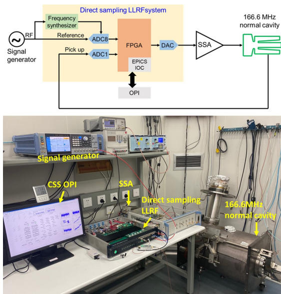
Figure 5: The LLRF test stand with a warm 166.6 MHz cavity.
