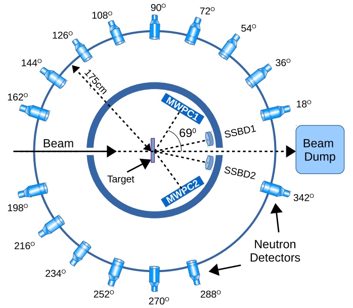
Fig. 1. (Color online) Experimental setup (top view) used for measurement of neutron multiplicity in coincidence with fission fragments. Two MWPCs, two monitor detectors (SSBD1 and SSBD2) and neutron detectors are placed in the reaction plane for ^{30}\text{Si} + ^{178}\text{Hf} .
