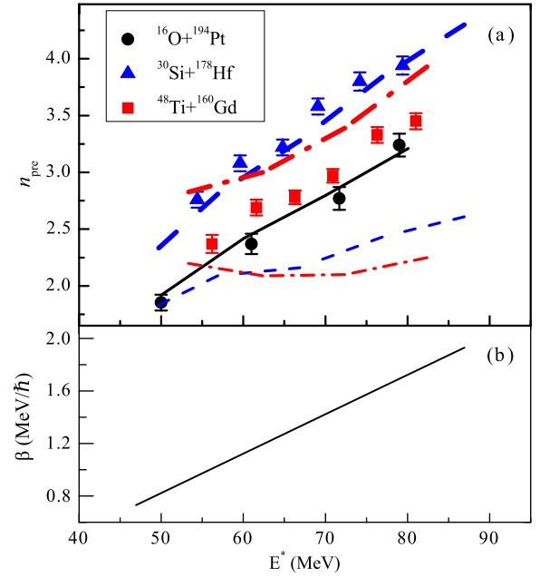
Fig. 6. (a) Measured n_{pre} for ^{30}\text{Si}+^{178}\text{Hf} (triangles), ^{48}\text{Ti}+^{160}\text{Gd} (squares), and existing data [29] for ^{16}\text{O}+^{194}\text{Pt} (circles) reactions. Thin lines are calculated n_{pre} for ^{30}\text{Si}+^{178}\text{Hf} (dashed lines), ^{48}\text{Ti}+^{160}\text{Gd} (dash-dotted lines), and ^{16}\text{O}+^{194} (solid lines) without formation delay. Thick lines correspond to \tau = 65 \times 10^{-21} s. The \beta used for the dynamical calculations is shown in (b).
