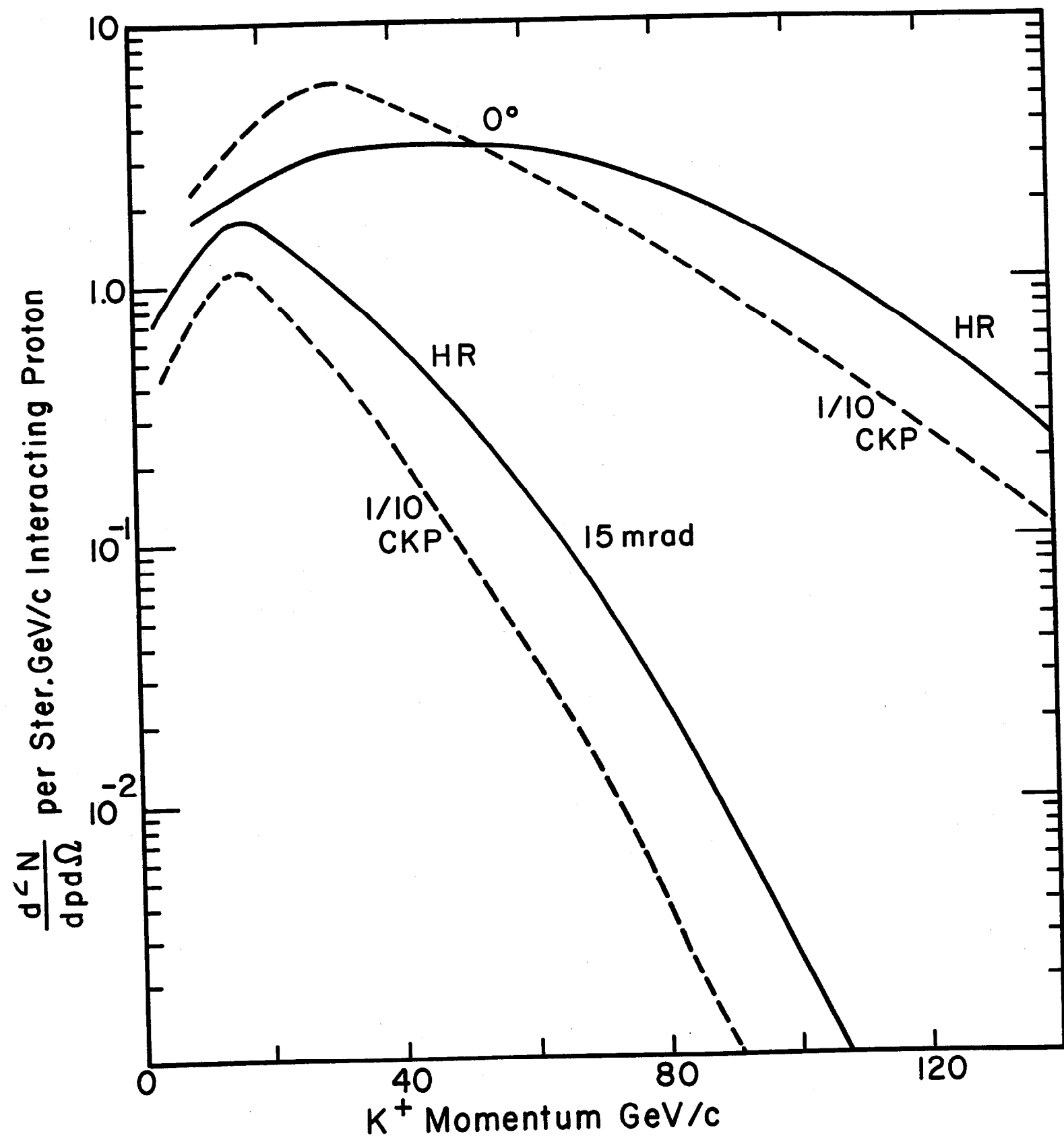
Fig. 3. K^+ yields at 0^\circ and 15 \text{ mrad} for 200-GeV p-p collisions according to 1/10 CKP and HR.
