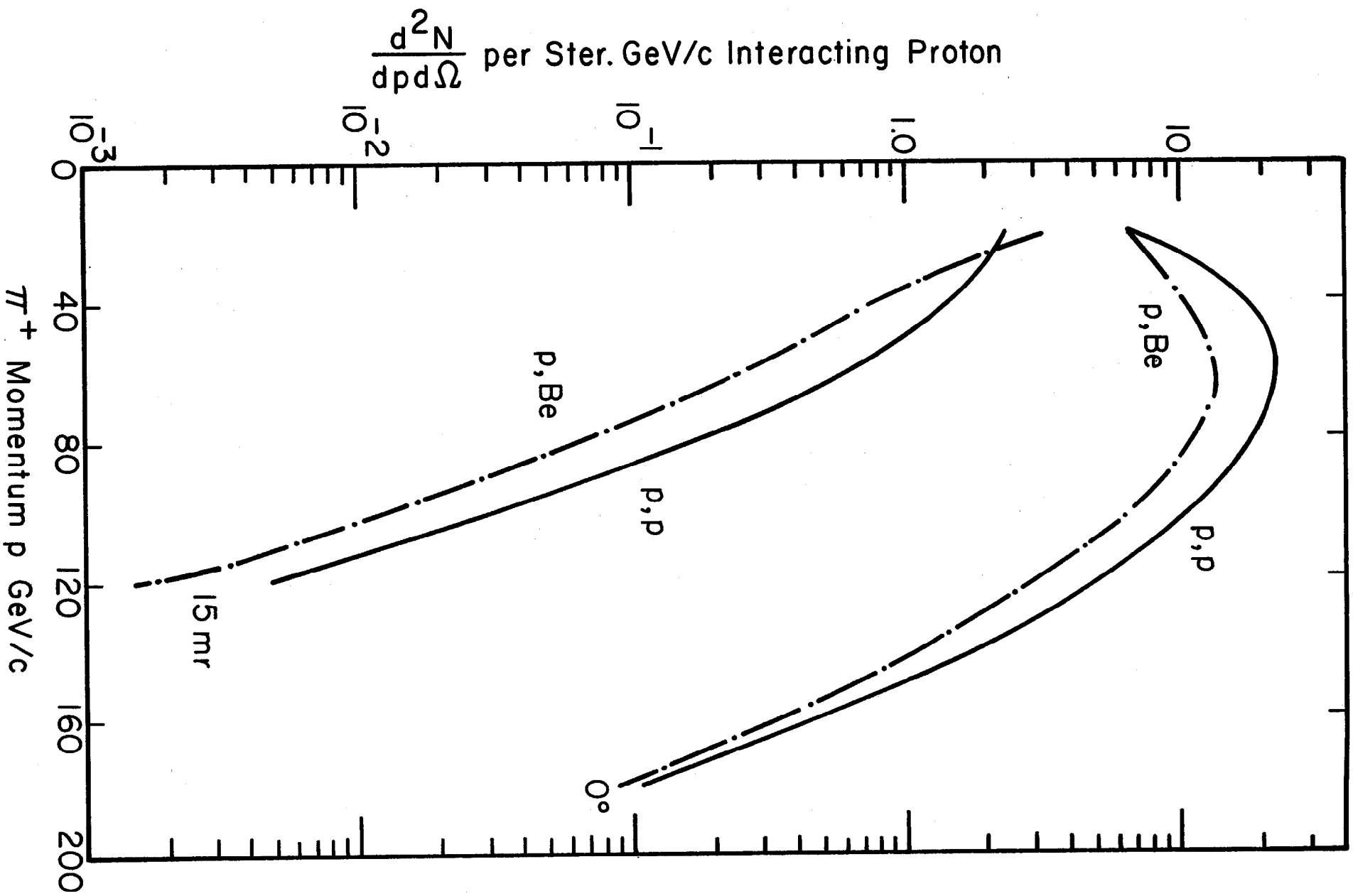
Fig. 15. \pi^+ yields at 0^\circ and 15\text{ mrad} according to the Trilling model
