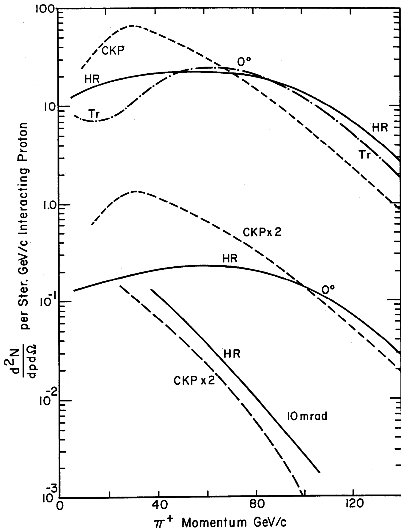
Fig. 1. \pi^+ yields at 0^\circ and 10 \text{ mrad} for 200-GeV proton-proton collisions
