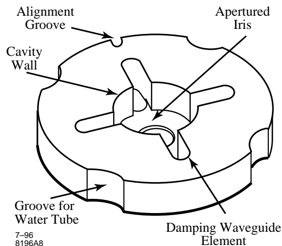
Figure 5. A cell of the Damped-Detuned structure.
