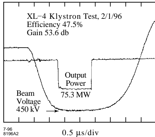
Figure 2. High-Power test of XL-4.
