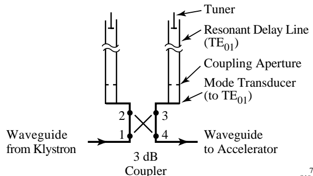
Figure 3. A schematic of the SLED-II rf compression.
