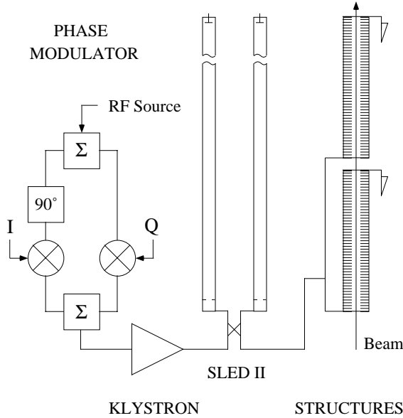
Figure 7. Layout of an RF station including the phase modulator which is controlled by the I & Q inputs.
