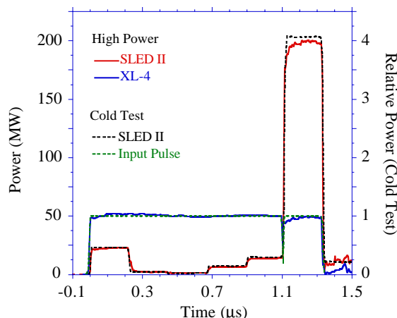
Figure 4. Test of Injector SLED-II system.
