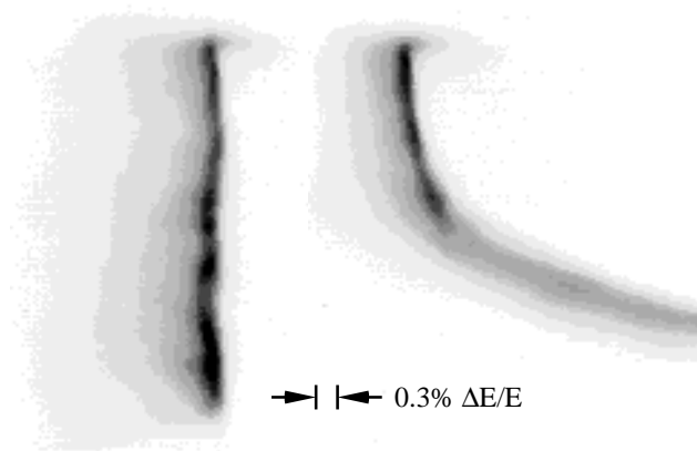
Figure 10. Profile monitor images of the bunch train at the end of the spectrometer. The kicker magnet has spread the 120 ns train length vertically with head of the train at the bottom. The dispersion generated by the spectrometer bend magnet has spread the electrons horizontally in proportion to their energy with higher energy toward the right. The left image was recorded with 13% loading compensation in the linac and right image with no linac compensation.
