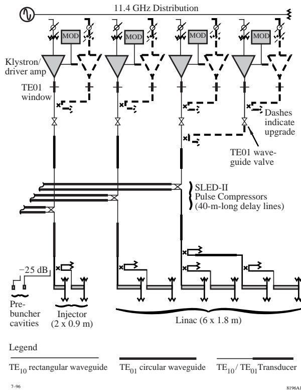
Figure 1. A schematic of the NLCTA rf system
