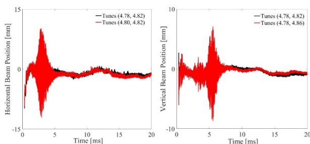
Figure 5: Measured beam positions over the whole time of 20-ms with different tunes.
