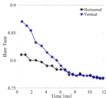
Figure 6: The measured tune variations during acceleration.
