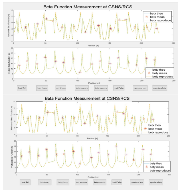
Figure 3: The comparison of the measured beta functions and the theoretical values at 1 ms (upper) and 10 ms (lower).
