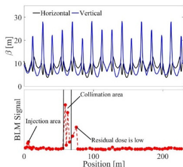
Figure 7: BLM signals along the RCS after the beam loss optimization.
