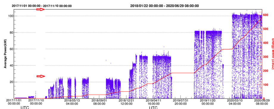
Figure 1: Beam power ramp-up history of CSNS/RCS, where the blue bars correspond to the beam power, while the red line shows the accumulated beam power.
