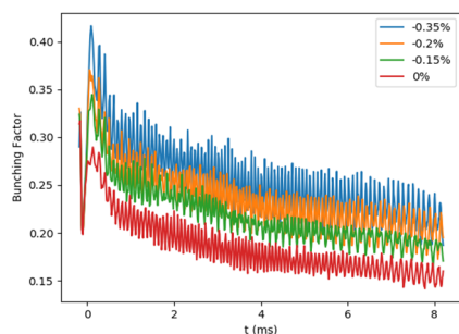
Figure 4: The measured bunching factor with different injection momentum offset.
