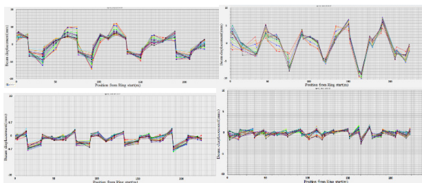
Figure 2: Measured COD on ring BPMs without (upper) and with (lower) the COD correction by the steering magnets, where 20 CODs are plotted for each at 1 ms regular intervals over the acceleration cycle (20 ms).
