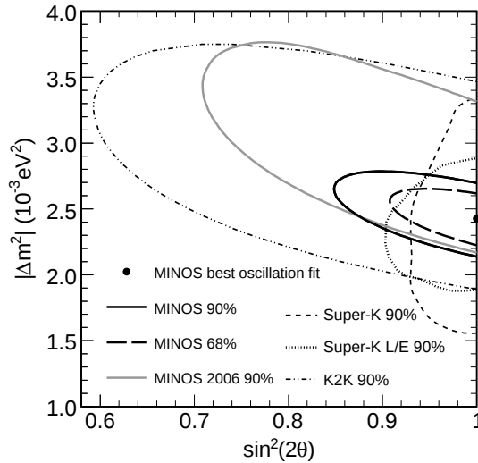
Fig. 1. Allowed regions for the mixing parameters \Delta m_{\text{atm}}^2 and \sin^2 2\theta_{23} for MINOS and K2K, compared to results from the Super-Kamiokande atmospheric experiment.
