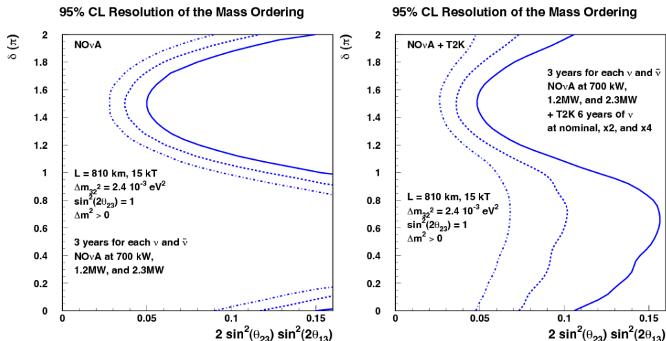
Fig. 2. NOvA/T2K sensitivity to the mass hierarchy. Left: 95% C.L. resolution of the mass hierarchy ( \text{sign}(\Delta m_{31}^2) ) as a function of \delta from NOvA neutrino and anti-neutrino running (normal hierarchy assumed). Right: the same plot for the combination of NOvA and T2K measurements. The lines denote three different assumptions for NOvA and T2K beam power. Plots courtesy [16].
