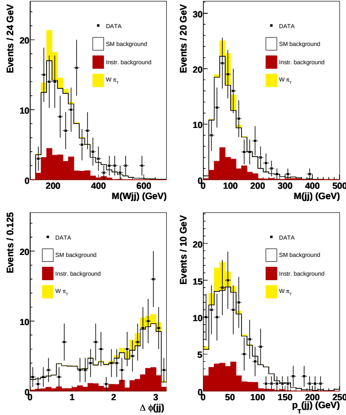
Fig. 1. Distribution for topological variables used for cut-based and NN analysis after Wjb selection. The white histogram represents the Standard Model prediction, dark (red) solid histogram represents the instrumental background, the light gray (yellow) histogram is the predicted W\pi_T signal for M(\rho_T) = 210 GeV and M(\pi_T) = 110 GeV. Black dots are data.
