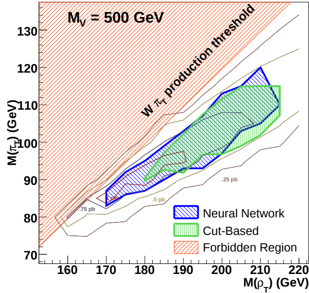
Fig. 3. Excluded region at 95% C.L. in the (M(\rho_T), M(\pi_T)) plane for \rho_T \rightarrow W\pi_T \rightarrow e\nu b\bar{b}(\bar{c}) production with M_V = 500 GeV calculated using 388 \text{ pb}^{-1} of D\bar{O} data with the cut-based analysis and with the neural network analysis. The diagonal line defines the kinematic threshold for W\pi_T production. The four iso-cross section curves indicate areas in the M_{\rho_T}, M_{\pi_T} plane where the expected cross section times branching ratio is \geq 1 \text{ pb} , \geq 0.75 \text{ pb} , \geq 0.5 \text{ pb} and \geq 0.25 \text{ pb} .
