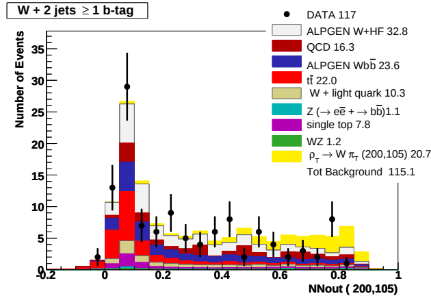
Fig. 2. Distributions of neural network output for signal and backgrounds. The top (yellow) histogram represents W\pi_T for M(\rho_T) = 200 GeV, M(\pi_T) = 105 GeV and M_V = 500 GeV.
