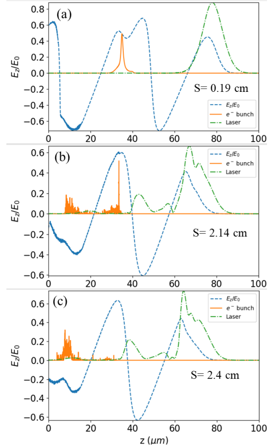
Figure 1: Beam spatial distribution (orange curve), net longitudinal wakefield (blue curve) and the laser envelope (green curve) at (a) s = 0.19 cm, (b) s = 2.14 cm (c) s = 2.4 cm, bunch moved toward the acceleration phase of wakefield.
