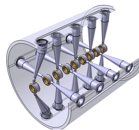
Figure 6: Model of the CCH1 dummy segment for welding and galvanic testing purposes.
