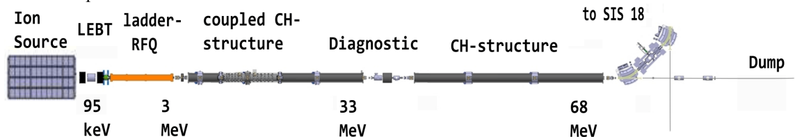
Figure 1: Layout of the FAIR Proton Linac.
