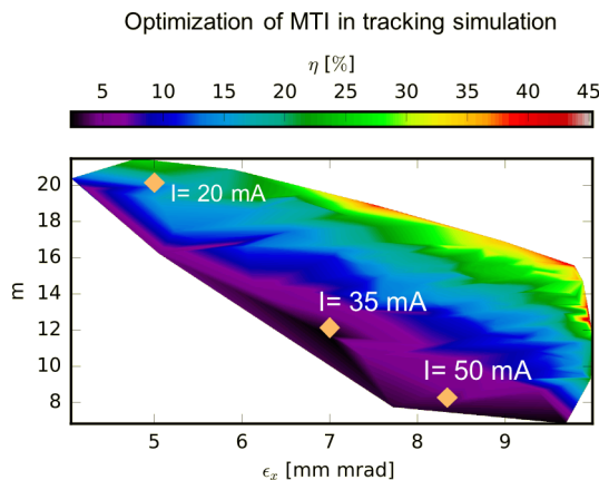
Figure 9: Proton linac MTI performance plot for the SIS18 synchrotron.
