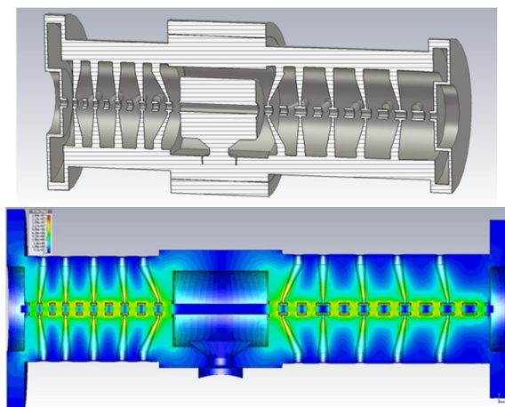
Figure 5: Layout of the first CCH-type cavity CCH1 and corresponding CST Microwave Studio calculations.
