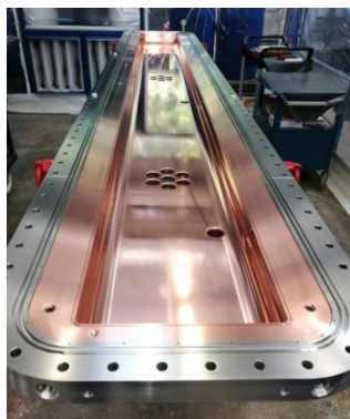
Figure 4: Copperplated RFQ half shelf at the GSI galvanic workshop.
