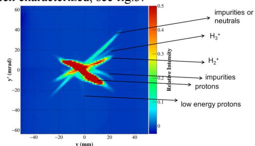
Figure 3: Typical emittance measurement taken at the diagnostic section within the LEBT.
