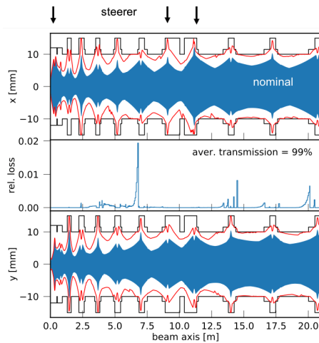
Figure 8: Simulated horizontal (upper) and vertical (lower) beam envelopes along the whole DTL section for a simulated current of 70 mA. In blue the nominal case, in red the overlap of all envelopes from all errors runs. Related loss (middle) along the DTL resulting from systematic error studies.
