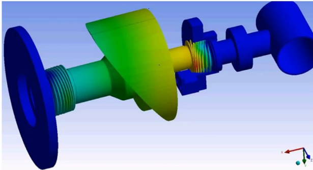
Figure 5: Mechanical model of the articulated FPC, showing the central DN100 6-inch conflat flange pair (middle of the figure). A section of beam pipe is shown in blue in the upper right side of the figure and the large insulating vacuum tank flange is shown on the left.
