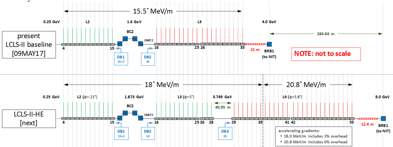
Figure 1: LCLS-II (top) and LCLS-II-HE (bottom) SRF linac layout schematic. (The injector and BC1 are omitted).
