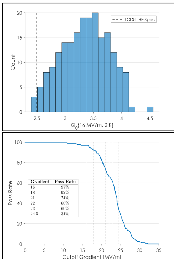
Figure 2: Cavity VT performance.
