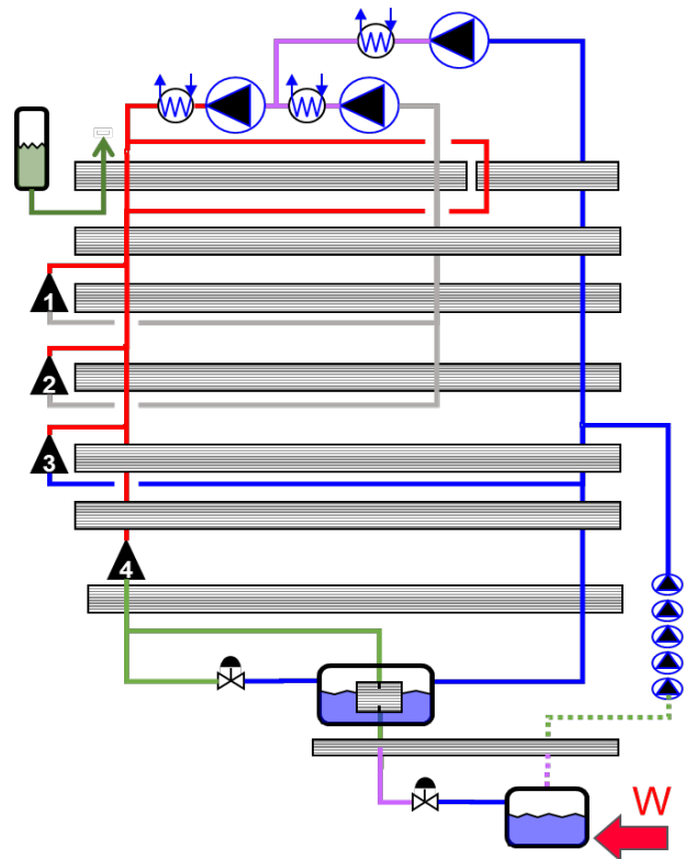
Figure 6: Single Cryoplant Process Flow Diagram, with room temperature at the top and 2K at the bottom. It shows the liquid nitrogen precooling (upper left), series/parallel high power warm compressors (top), expansion turbines (left), cold-box heat exchangers (8 each), sub-cooler vessel and heat exchanger, JT expansion valves (bottom, one in the cryoplant and one in CM), cold compressors (lower right). The cavity tanks are shown in the lower right with a red W to indicate heat from SRF.
