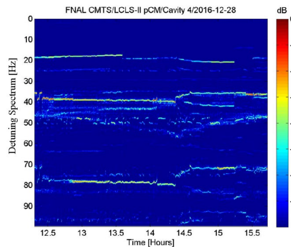
Figure 4: showing a four-hour duration cavity detuning spectrogram (difference between the cavity resonant frequency and nominal center frequency). The slow frequency drifts are correlated with the movement of cryogenics in the cryomodule and are consistent with TAO-generated frequencies.
