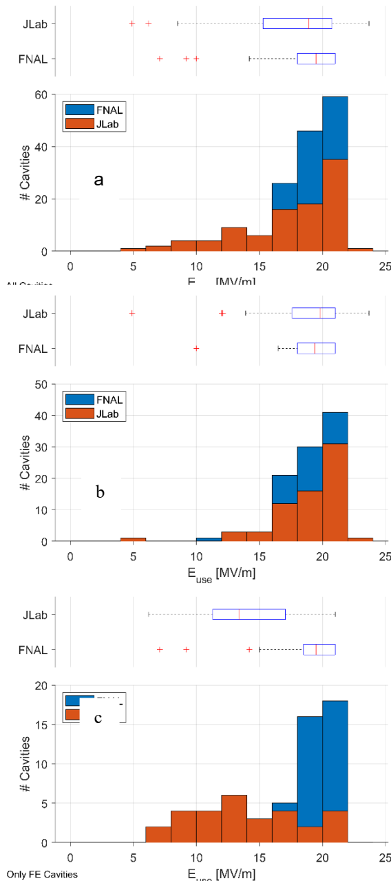
Figure 3: E_{acc} (usable) in CM test for a) all CM, b) no FE, c) only FE cavities. (The bins are overlaid).
