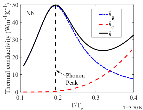
Figure 1: Phonon and electron contributions to the thermal conductivity of undeformed superconducting Nb.
