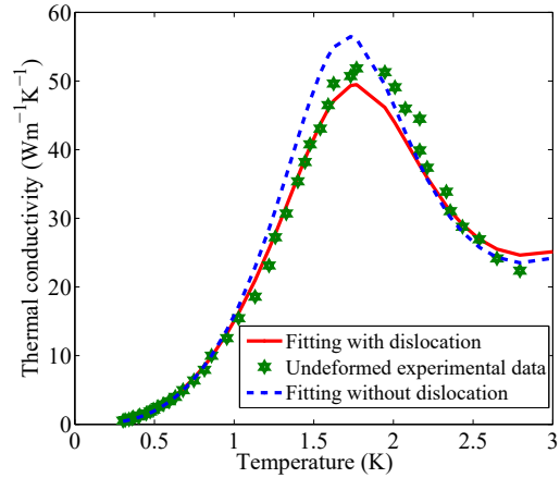
Figure 3: Comparison between fitting with or without dislocation term for undeformed Nb sample from [3]. Calculated dislocation density is N_d = 4.7 \times 10^{12} \text{ m}^{-2} .
