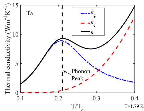
Figure 2: Phonon and electron contributions to the thermal conductivity of undeformed superconducting Ta.
