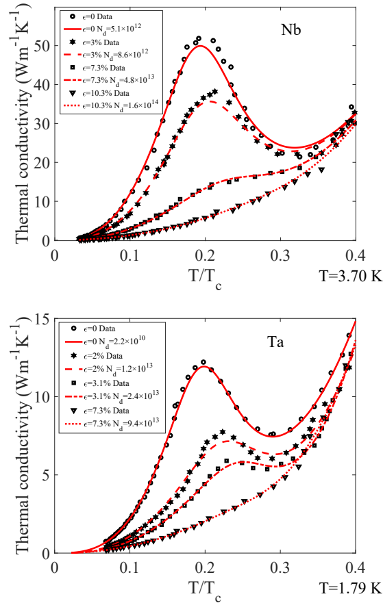
Figure 5: Comparison between the data of the thermal conductivity of deformed superconducting metals (symbols) and the best fit using Eq. (1) (lines). Top panel is Nb [3], for \epsilon = 0\% , 3\% , 7.3\% , and 10.3\% and bottom panel is Ta [7], for \epsilon = 0\% , 2\% , 3.1\% , and 7.3\% . The dislocation density is calculated during the fitting process
