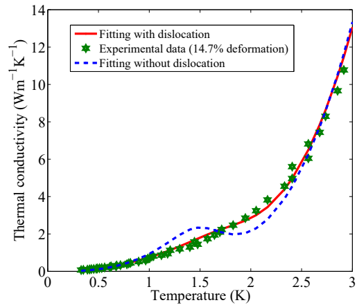
Figure 4: Comparison between fitting with or without dislocation term for deformed Nb sample [3]. Calculated dislocation density is N_d = 3.8 \times 10^{14} \text{ m}^{-2} .
