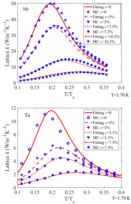
Figure 7: Monte Carlo solution of Eq. (4) (symbols) compared with the best fit of Eq. (1) (lines) for the lattice thermal conductivity of deformed sample Nb3 [3] (top panel) with \epsilon = 0\% , 3%, 7.3%, and 10.3% and deformed sample Ta1 [7] (bottom panel) with \epsilon = 0\% , 2%, 3.1%, and 7.3%. The parameters (size, RRR, deformation temperature, and estimated N_d ) for each sample are listed in Table 1.
