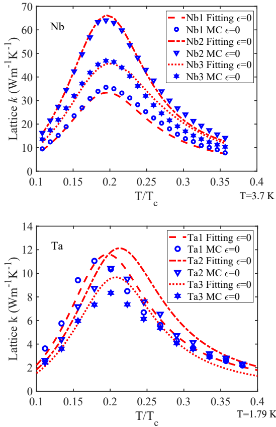
Figure 6: Monte Carlo solution of Eq. (4) (symbols) compared with the best fit of Eq. (1) (lines) for the lattice thermal conductivity of three undeformed Nb samples [3] (top panel) and three undeformed Ta samples [7] (bottom panel). The parameters (size, RRR, deformation temperature, and estimated N_d ) for each sample are listed in Table 1.
