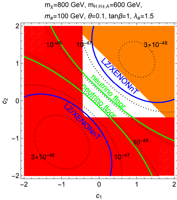
Figure 1. The contours of \sigma_{\text{SI}} [ \text{cm}^2 ] for m_\chi = 800 GeV. The blue solid lines show the LZ and XENONnT prospects [17, 18], We take m_{H,H^\pm,A} = 600 GeV, m_a = 100 GeV, \theta = 0.1 , \tan\beta = 1 , and \lambda_a = 1.5 . The region between two green lines is below the neutrino floor [20]. The global minimum does not break the electroweak symmetry in the orange shaded region. In the red shaded region, the scalar potential is unbounded from below.
