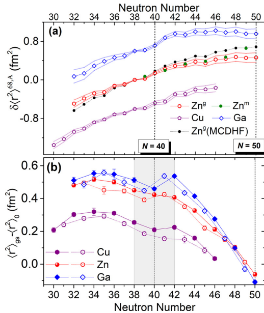
Fig. 1. (a) Changes in mean square charge radii for the Zn isotopes compared with neighbouring Cu and Ga isotopic chains, which are vertically offset by \pm 0.6 fm 2 for clarity. The black dots present the Zn radii extracted by using the K_{\text{MS}} from MCDHF calculations. (b) Experimental \langle r^2 \rangle for ground states of the Cu, Zn and Ga isotopes with the spherical volume contribution \langle r^2 \rangle_0 from the droplet model subtracted [21].
