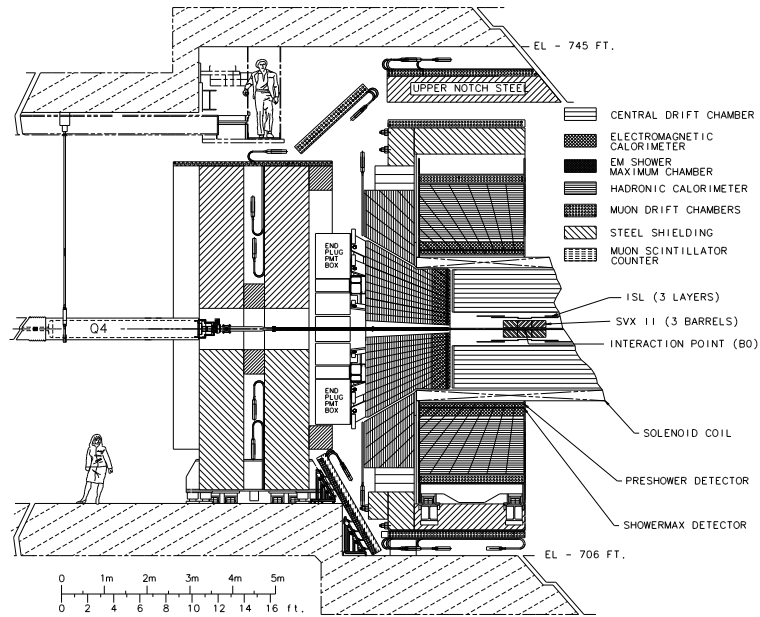
Fig. 6. CDF detector
