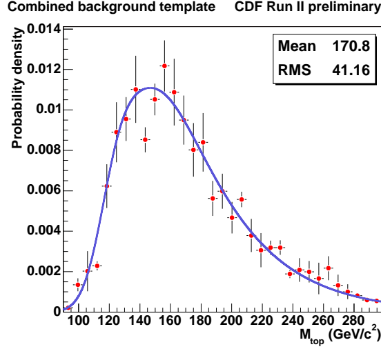
Fig. 19. Distribution of raw top mass for background treated as t\bar{t} signal
