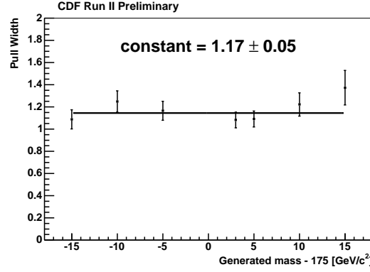
Fig. 28. Pull width dependence as a function of input top mass
