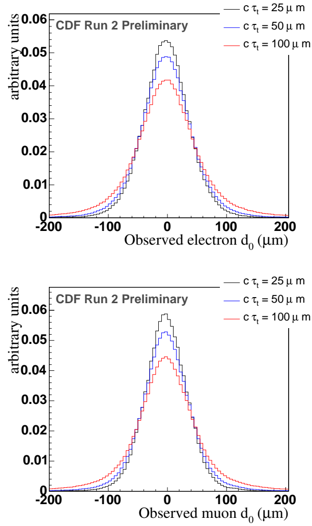
Fig. 53. Templates for t\bar{t} signal simulated for different top lifetime electron and muon tracks impact parameter distribution.
