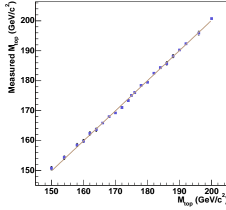
Fig. 20. Test of the top mass reconstruction procedure by pseudo-experiments.
