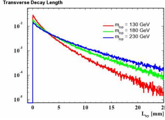
Fig. 17. Distribution of transverse decay length for top mass 130,180,230 GeV/ c^2
