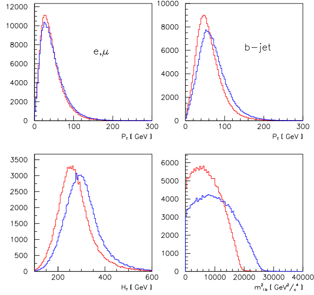
Fig. 16. Distribution of several variables sensitive to top mass. P_T of e, \mu from top decay chain (W), P_T of b-jets, H_T and quadrature of effective mass of lepton and b-jet m^2_{lb} . In red color distributions represent top mass 160 GeV/ c^2 , in blue top mass 180 GeV/ c^2
