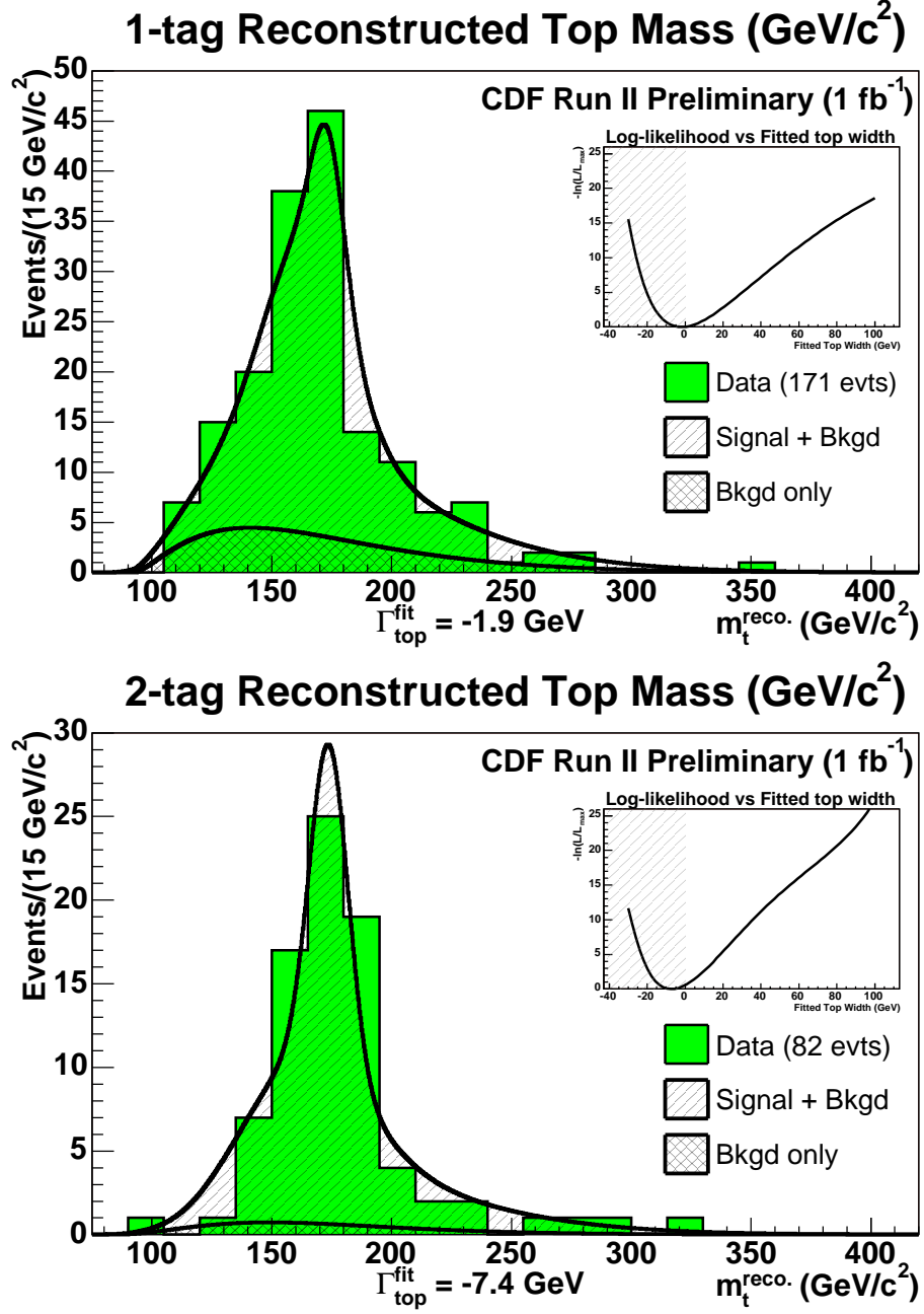
Fig. 58. Likelihood fit of top width to reconstructed top mass distribution of data. Upper plot for 1-b-tagged sample, lower plot for 2-b-tagged sample.
