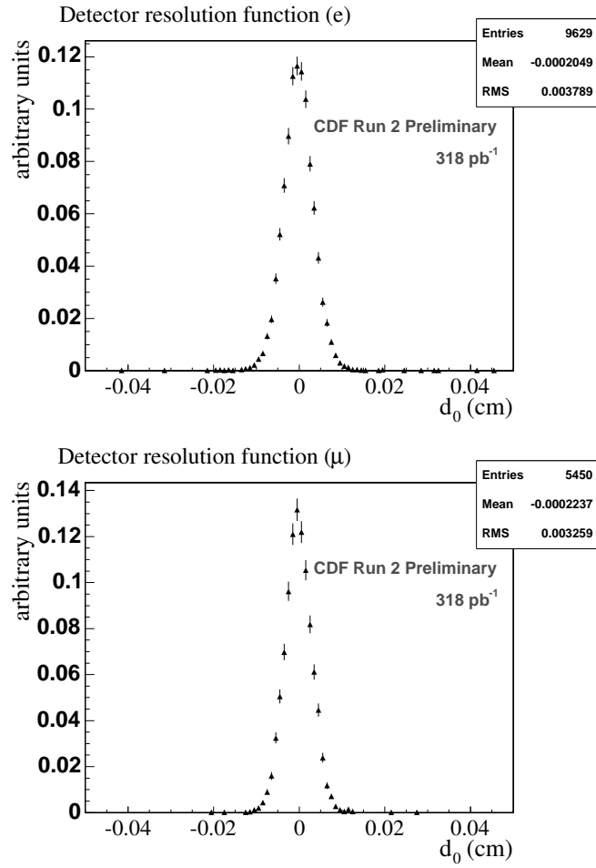
Fig. 51. impact parameter resolution for isolated electrons and muons from Z^0 decay
