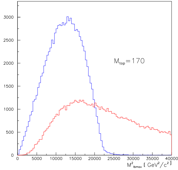
Fig. 39. Distribution of max M_{lb}^2 for correct pairing (blue) and wrong pairing (red)
