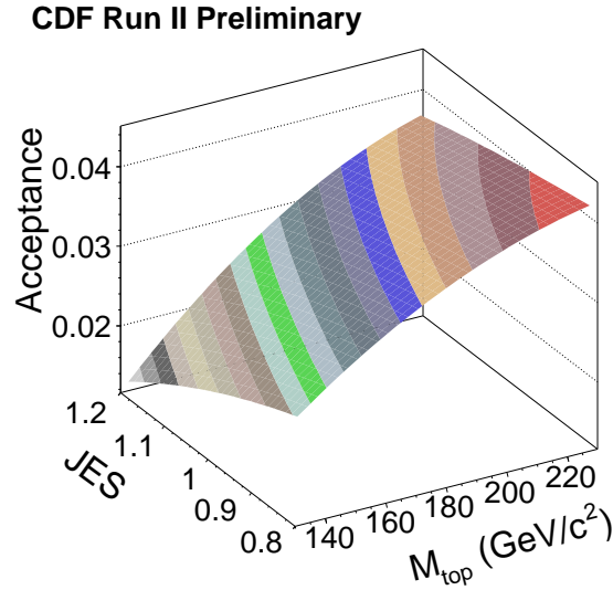
Fig. 24. Acceptance dependence as a function of JES and top mass
