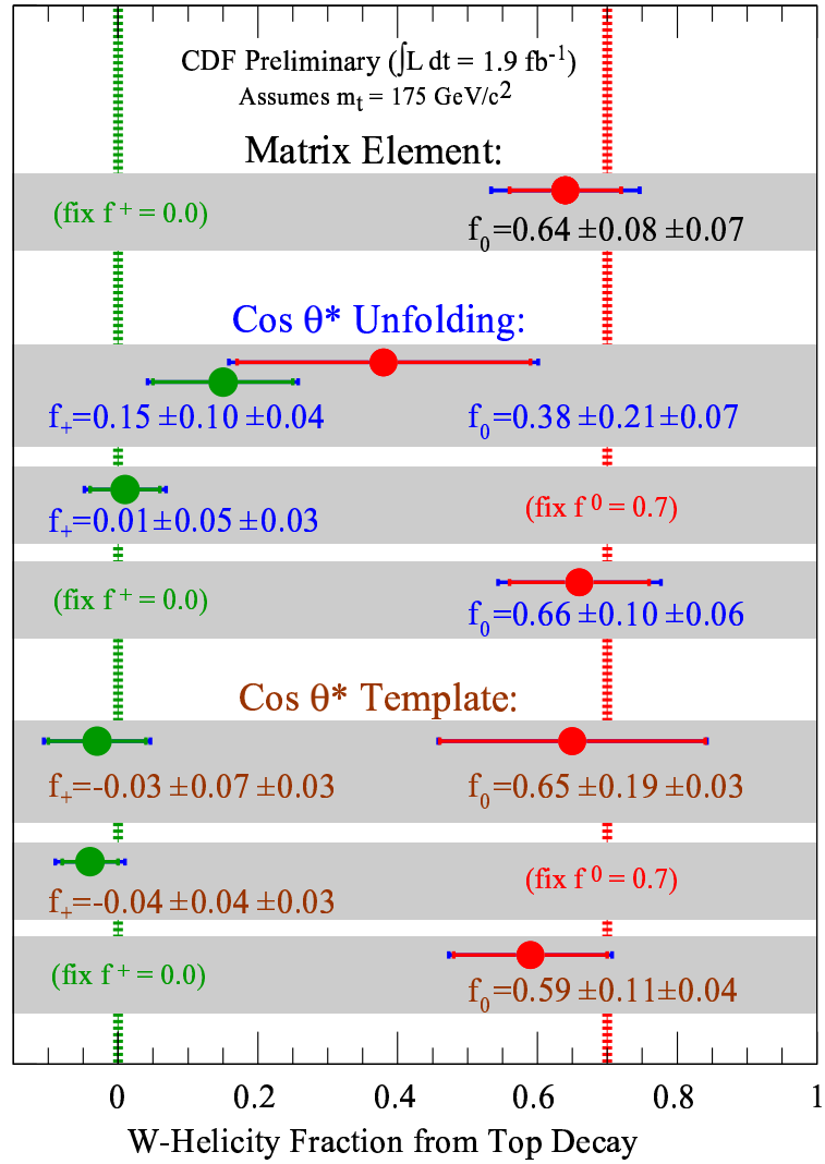
Fig. 46. Summary of the results of CDF collaboration on W helicity fraction measurement
