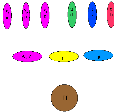
Fig. 1. Structure of fundamental blocks of matter.
