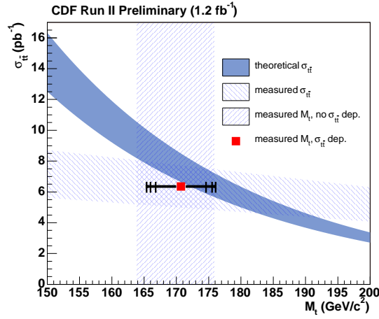
Fig. 23. Top mass measurements by combination of kinematics and cross section measurement. The blue solid bands shows theoretical t\bar{t} cross section within its uncertainties. Hatched areas mark the cross section measurement as a function of top mass and independent top mass measurement based on kinematics and templates (see Fig. 21). Red square with error bars mark the measured top mass by combined cross section and kinematics method (see text).
