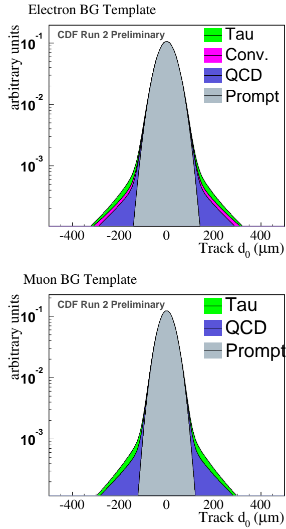
Fig. 52. Influence of different kind of background on impact parameter distribution for electron and muon tracks
