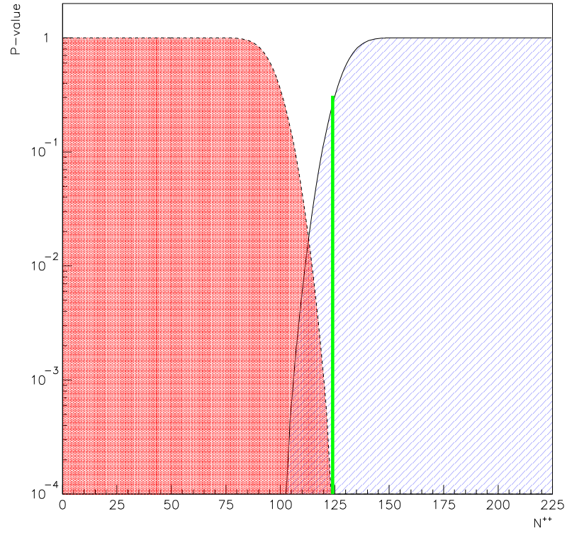
Fig. 42. Probability to observe N^{++} pairs or less supporting SM top if SM hypothesis is true - blue curve (region) and complementary case when exotic hypothesis (XM) is correct. Probability to correctly determine top charge was set to P_s = 0.572
