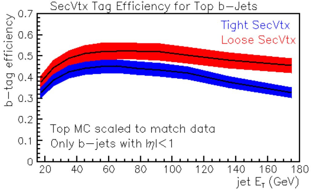
Fig. 11. Tagging efficiency for a “tight” and “loose” version of SecVtx algorithm as a function of E_T of b-jets
