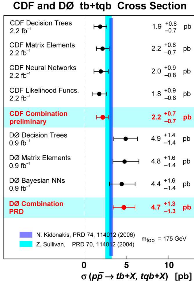
Fig. 36. Summary of measurements of single top cross section by DØ and CDF collaboration
