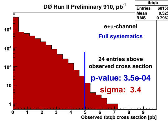
Fig. 35. Test of procedure of measurement cross section on background-only pseudo-datasets
