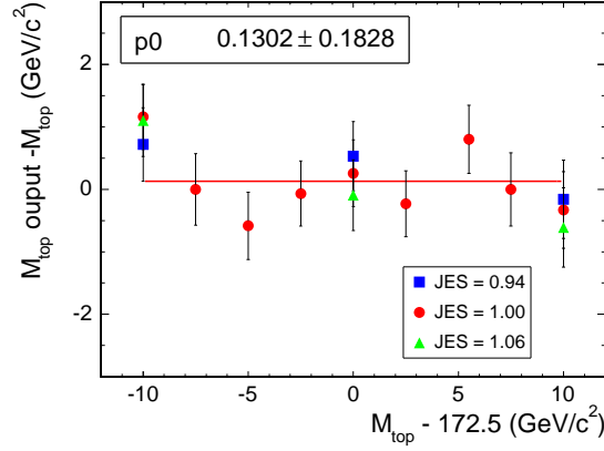
Fig. 26. Linearity check of reconstructed top mass as a function of input top mass for 83% of signal and 17% of background. Input JES was fixed at 0.94, 1.0 and 1.06 values
