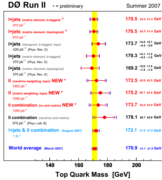
Fig. 31. Summary of top mass measurements by the collaboration DØ
