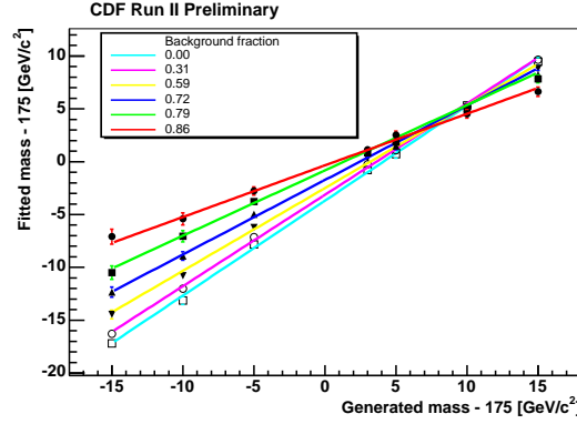
Fig. 27. Calibration curves for dependence of fitted top mass as a function of input top mass for different background fractions
