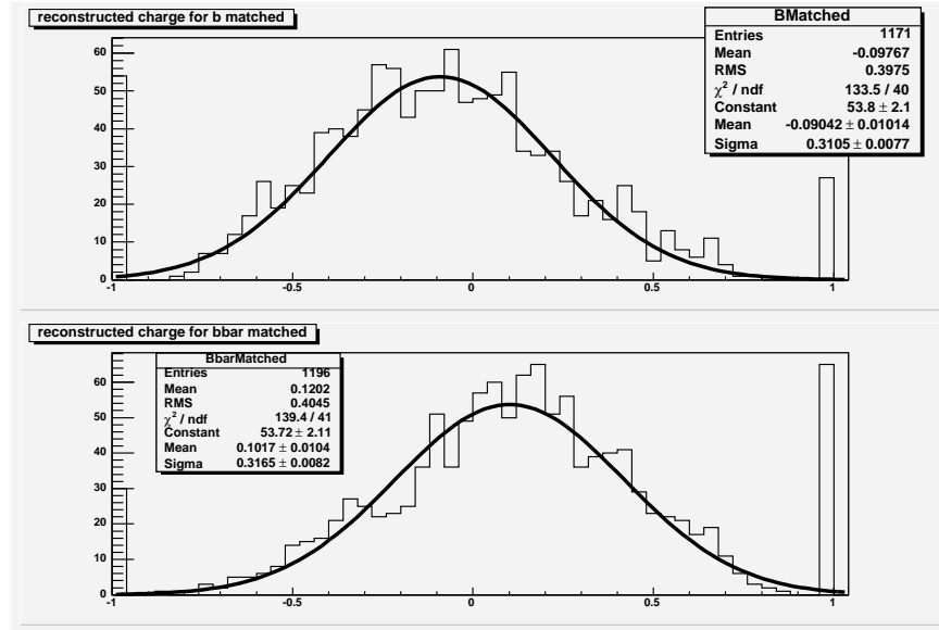
Fig. 38. Charge distribution for matched b-jets (upper plot) and \bar{b} -jets
