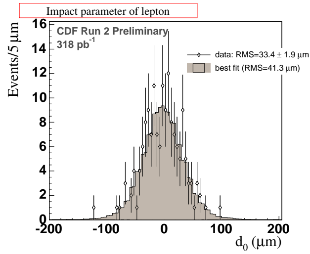
Fig. 54. A comparison of impact parameter distribution of leptons for t\bar{t} candidates and best fit by templates
