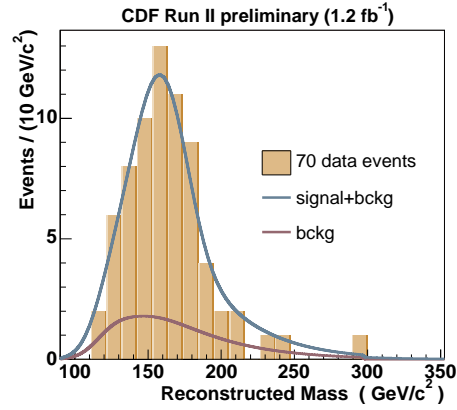
Fig. 21. Top mass fit to data
