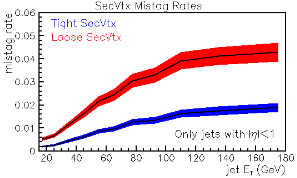
Fig. 12. Miss-tag probability for a “tight” and “loose” version of SecVtx algorithm as a function of E_T of b-jets
