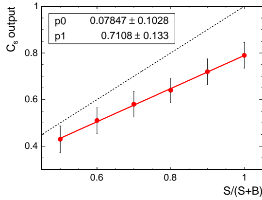
Fig. 25. Dependence of fitted output signal fraction C_s as a function of input signal fraction S/(S+B) and a comparison with an ideal case
