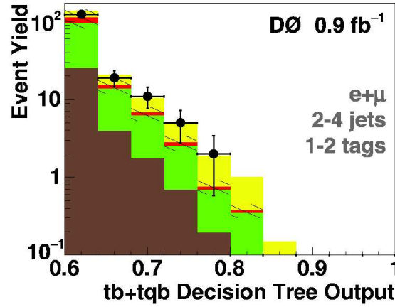
Fig. 33. Distribution of output from boosted decision tree for sum of all 12 channels for tb+tqb search. Different colors represent different contribution: green - W+jets, brown - multi-jets, red - t\bar{t} and yellow - single top scaled according to measured cross section
