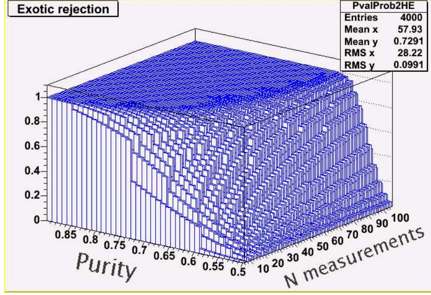
Fig. 37. Two dimensional distribution of probability to reject “wrong” hypothesis at 95% CL as a function of purity and number of measurements
