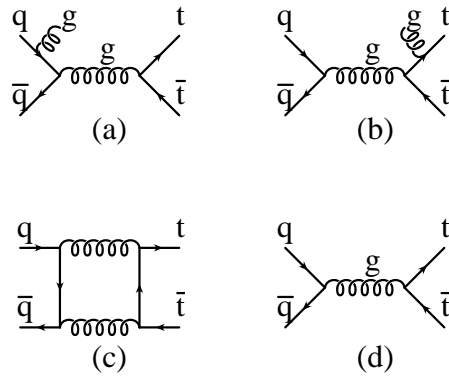
Fig. 5. Interference of diagrams (a) and (b), (c) and (d) has a consequence in forward backward asymmetry for top quark production
