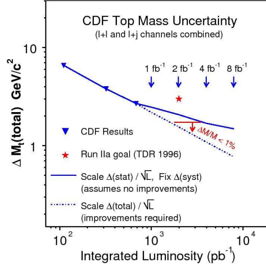
Fig. 29. Expected total top mass error (systematic and statistical added in quadrature) dependence as a function of accumulated statistics (for more detail see text)
