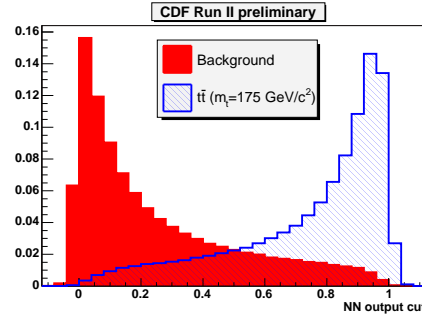
Fig. 13. Response of trained ANN to t\bar{t} signal and background
