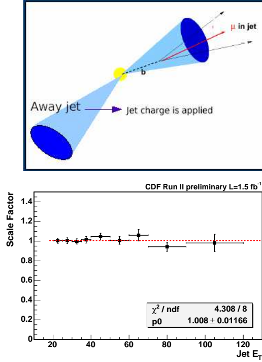
Fig. 40. Idea for determination b-jet charge purity from enhanced b-dijet data (upper picture) and dependence of scale factor as a function of b-jet E_T
