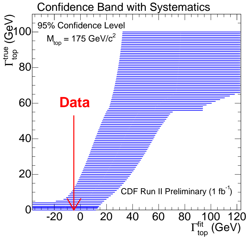
Fig. 59. Feldman-Cousins 95% Confidence Level bands. Mapping of fitted top width values to the range of corresponding true top width.
