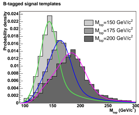
Fig. 18. Distribution of raw top mass for templates for b-tagged templates for top mass 150, 175 and 200 \text{GeV}/c^2
