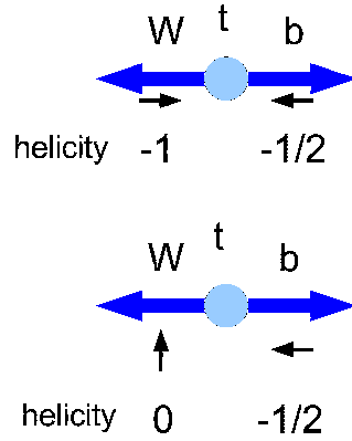
Fig. 43. Decay of top quark into W and b in top rest frame. Upper part represents top spin projection +1/2, W helicity -1 and b-quark helicity -1/2 (both left-handed), Lower part represents top spin projection -1/2, W helicity 0 (longitudinal) and b-quark helicity -1/2 (left-handed)
