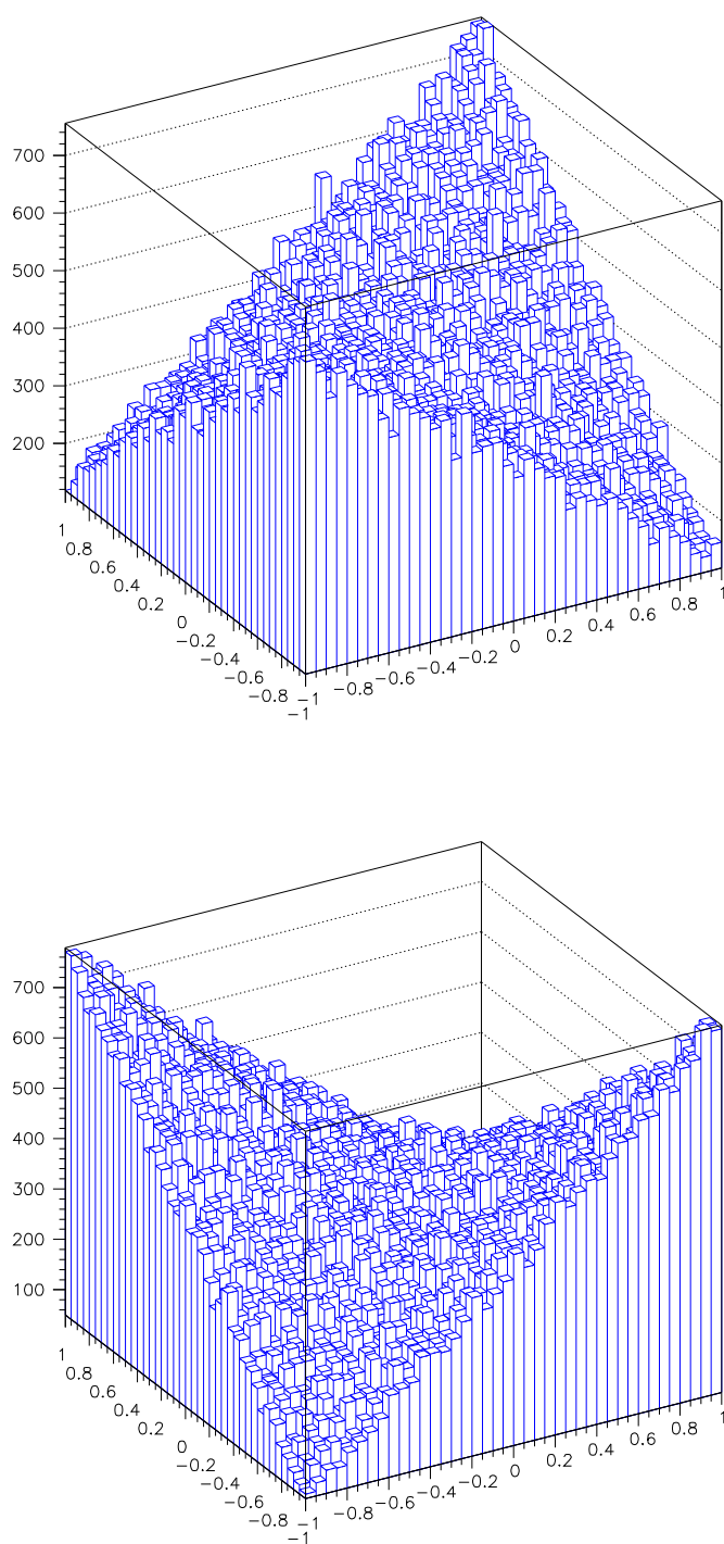
Fig. 48. A two dimensional distribution of \cos(\theta_1) \times \cos(\theta_2) in beam frame I (upper plot) and beam frame II (lower plot) - TopRex
