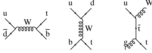
Fig. 4. Feynman diagrams for single top quark production
