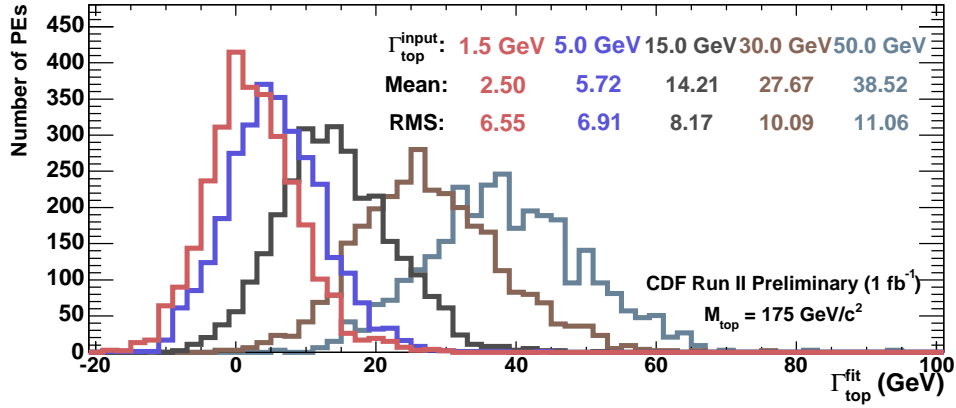
Fig. 57. Fitted width distribution for 3000 pseudo-experiments using MC samples with various \Gamma_t^{input}
