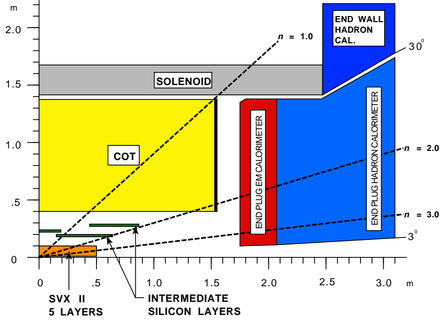
Fig. 7. Longitudinal view of CDF tracking system
