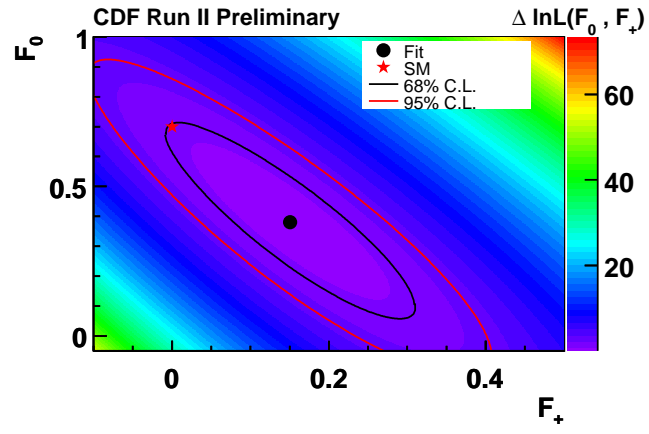
Fig. 45. \Delta \ln L dependence as a function of F_+ , F_0 around fitted value (black point). Position of SM predicted value for F_+ , F_0 is marked by red star. The black line indicate 68% CL contour, red one 95% CL.
