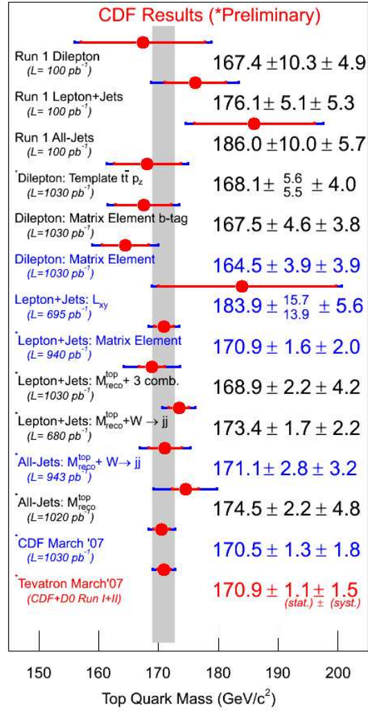
Fig. 30. Summary of top mass measurements by the collaboration CDF
