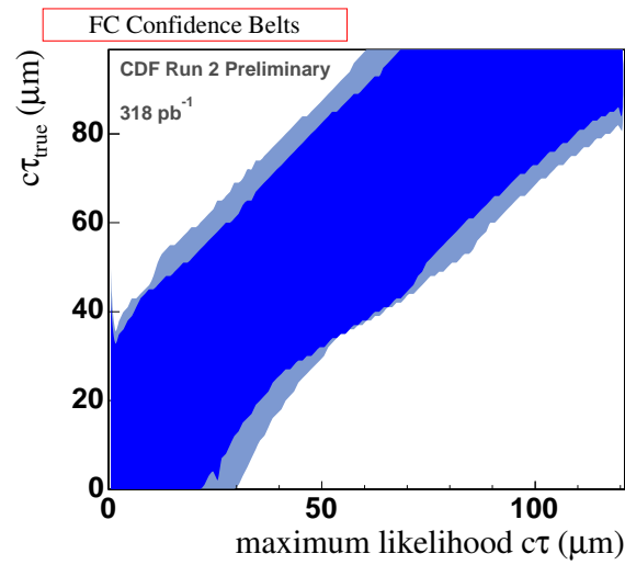
Fig. 55. Feldman-Cousins confidence level bands between measured and true top c\tau measurement
