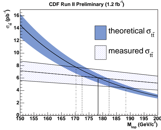
Fig. 22. Extraction of top mass from top mass dependence of theoretical cross section and top mass dependence of measured cross section
