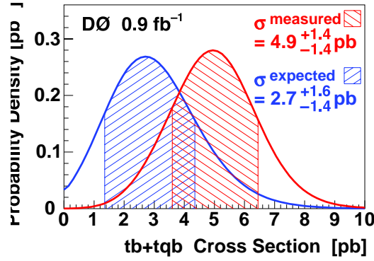
Fig. 34. Expected SM and measured Bayesian posterior probability densities for the tb + qtb cross section. Shaded lines indicate 1 standard deviation above and below peak positions.
