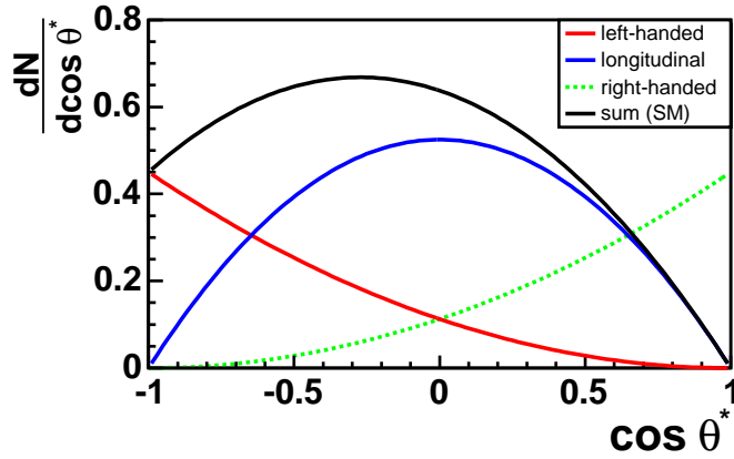
Fig. 44. Expected angular distribution of leptons in W rest frame in case W_- , W_0 , W_+ helicity states compared to SM expectation
