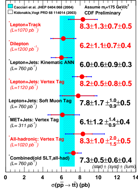
Fig. 14. Measurement of t\bar{t} production cross section by CDF collaboration
