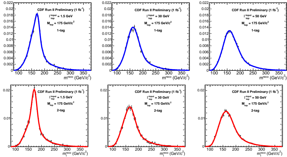
Fig. 56. Parametrization fits to the reconstructed top mass distributions for \Gamma_t^{\text{input}} 1.5, 30, and 50 GeV. Top: 1-b-tag sample, Bottom: 2-b-tag sample.
