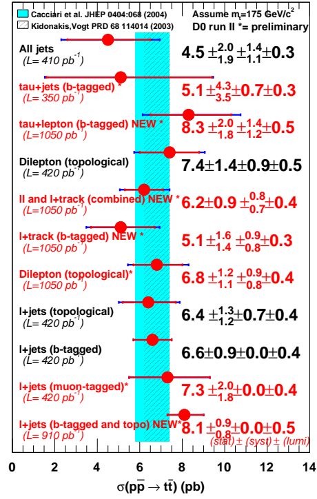
Fig. 15. Measurement of t\bar{t} production cross section by D0 collaboration
