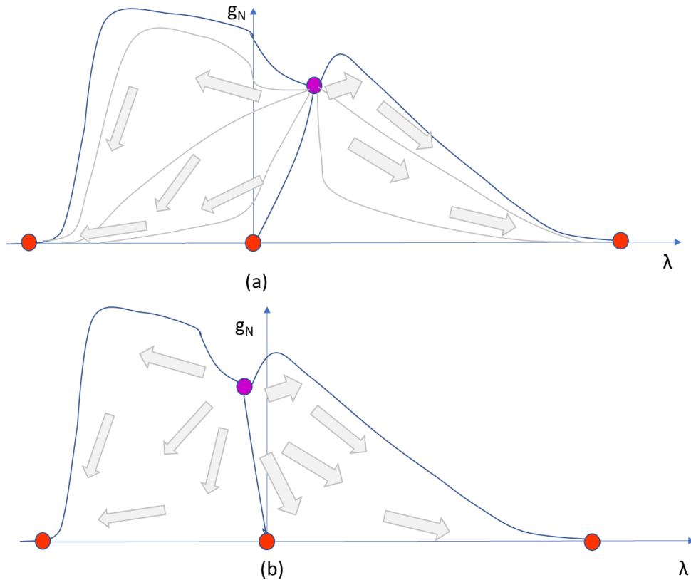
Figure 1: It illustrates the general forms of the UV critical curves as a (\lambda, g_N) phase diagram per the non-perturbative reasoning presented in this paper (conventional Physics). This is for a situation, where no matter or fields are present. (a) correspond to a positive \lambda at the UV fixed point while (b) corresponds to a negative one. Violet circle marks the UV fixed point. Red circles are IR fixed point. They are assumed to exist. A multi-fold reasoning renders (a) more probable while a superstrings origin would force a (b) diagram. In the presence of matter or fields, the diagrams are modified (typically and deformed to the left (UV point moving to the left until it (possibly) can't exist anymore). These diagrams are to be compared to the results of actual computations as done in Figure 4 of [38].
