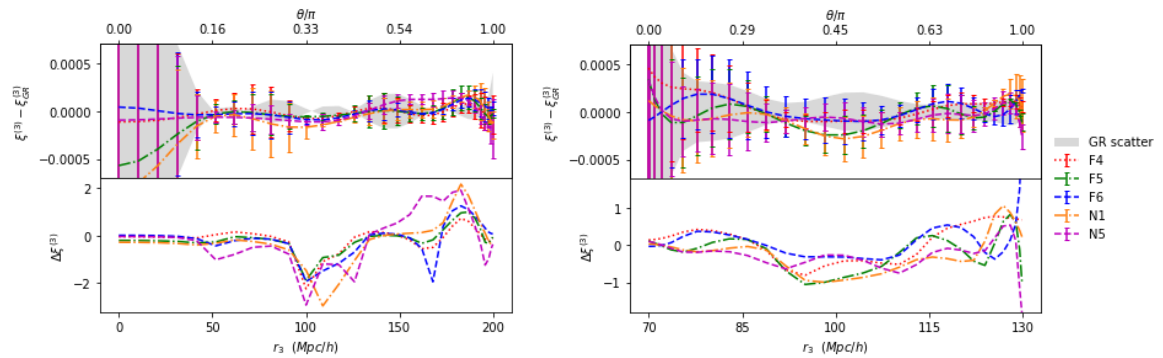
Figure 20. Full 3PCFs for r_1 = 100h^{-1}\text{Mpc} and r_2 = r_1 ( Left ) or r_2 = 30h^{-1}\text{Mpc} ( Right ). The top panels show differences of the MG 3PCF with respect to GR as a function of the third triangle side r_3 , or equivalently, the opening angle \theta_{12} between r_1 and r_2 . The bottom panels show the model differences using the analog of the variable \Delta\sigma\xi_\ell^{(3)} but for the full 3PCF. We use the first \ell < 10 multipole moments in figure 19 to construct the complete 3PCF.
