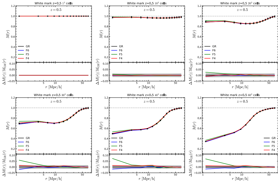
Figure 33. (Color Online) The marked correlation functions (mCF) with the White mark with (\rho_*, p) = (4, 10) , for different numbers of cells used to calculate the density field.
