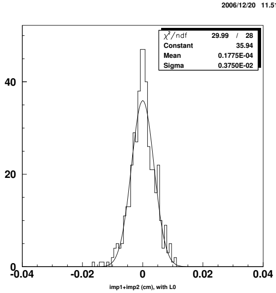
Fig. 6. Impact parameter resolution for tracks with a hit in Layer 0 and p_T < 5 GeV/c from cosmic muon data. Sigma of the Gaussian in the plot should be multiplied by 1/\sqrt{2} .
