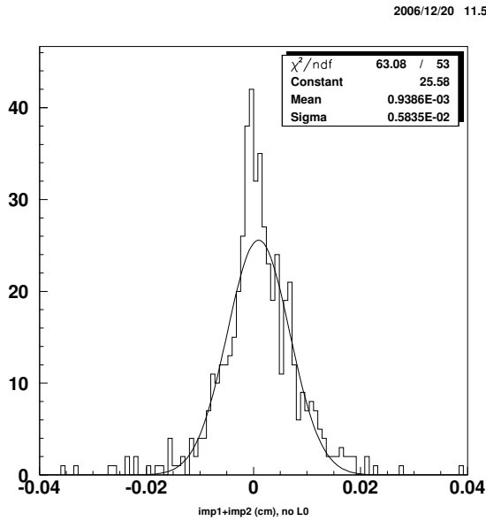
Fig. 7. Impact parameter resolution for tracks without a hit in Layer 0 and p_T < 5 GeV/c from cosmic muon data. Sigma of the Gaussian in the plot should be multiplied by 1/\sqrt{2} .
