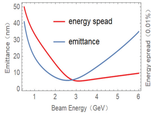
Figure 9: The emittance and energy spread evolution.
