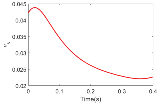
Figure 5: synchrotron tune curve in ramping process.
