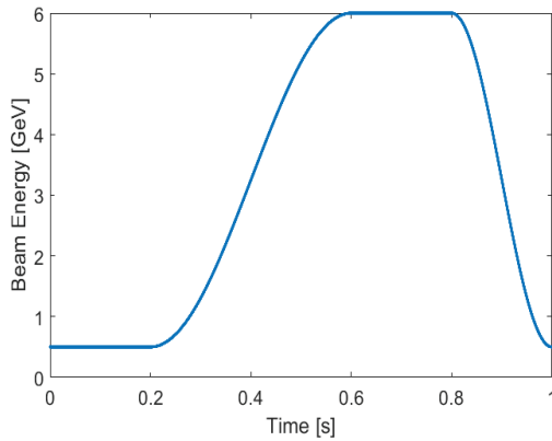
Figure 3: An energy ramp cycle of HEPS booster.
