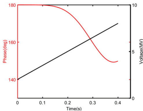
Figure 4: The synchrotron phase changes with RF voltage. Red line: synchrotron phase; Black line: RF voltage.
