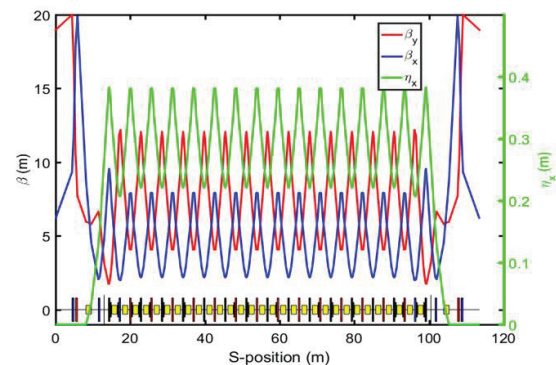
Figure 2: The optical functions and lattice structure of one quarter of the booster.
