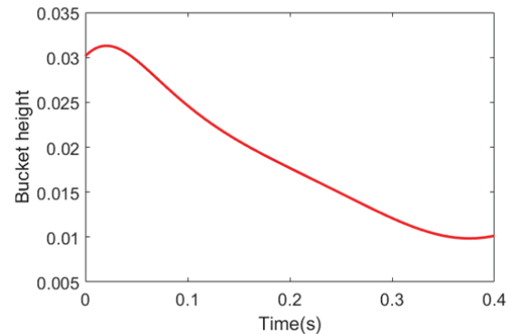
Figure 6: Bucket height changes in ramping up process.
