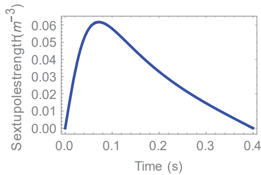
Figure 7: The sextupole strength induced by eddy current in ramping up process.
