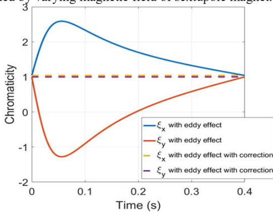
Figure 8: Eddy current induced chromaticity change.
