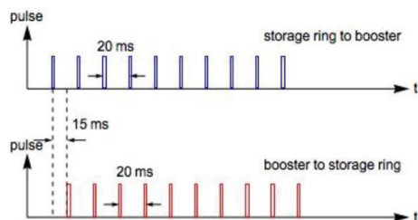
Figure 1: The time structure of bunches in two high energy transport lines.
