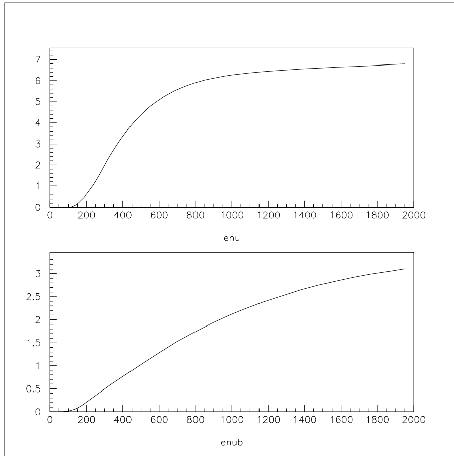
Figure 7.1: The cross sections (in units of 10^{-38} cm 2 ) for \nu_e C \rightarrow e^- N and \bar{\nu}_e C \rightarrow e^+ B quasi-elastic scattering as a function of incident neutrino energy in MeV.
