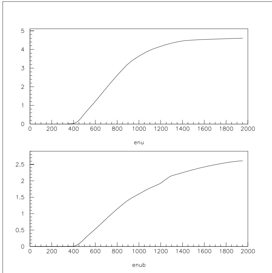
Figure 7.7: The cross sections (in units of 10^{-38} \text{ cm}^2 ) for \nu_\mu C and \bar{\nu}_\mu C charged current pion production as a function of incident neutrino energy in MeV.
