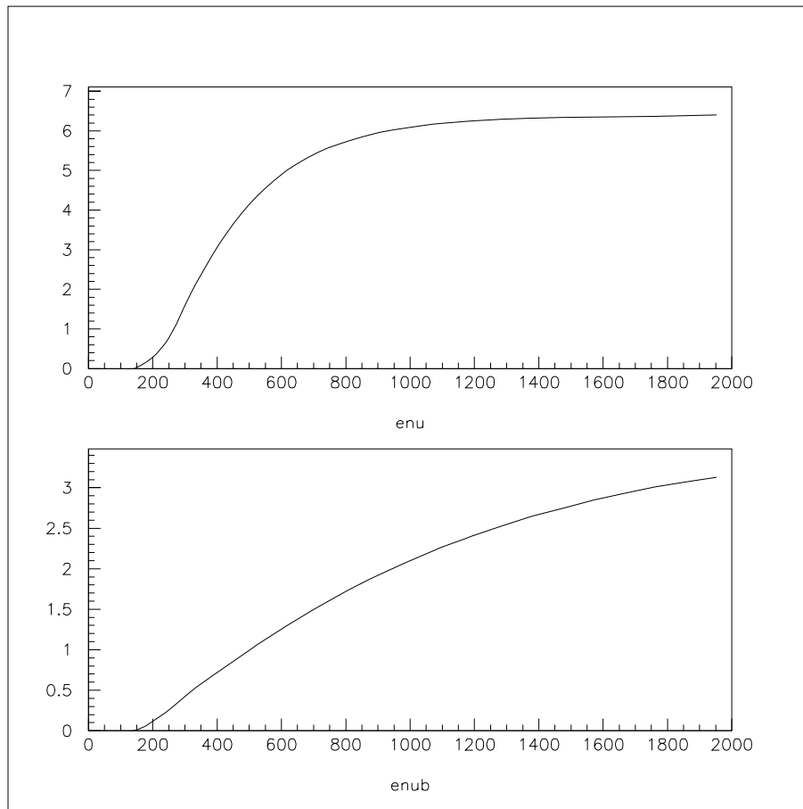
Figure 7.4: The cross sections (in units of 10^{-38} \text{ cm}^2 ) for \nu_\mu C and \bar{\nu}_\mu C quasi-elastic scattering as a function of incident neutrino energy in MeV.
