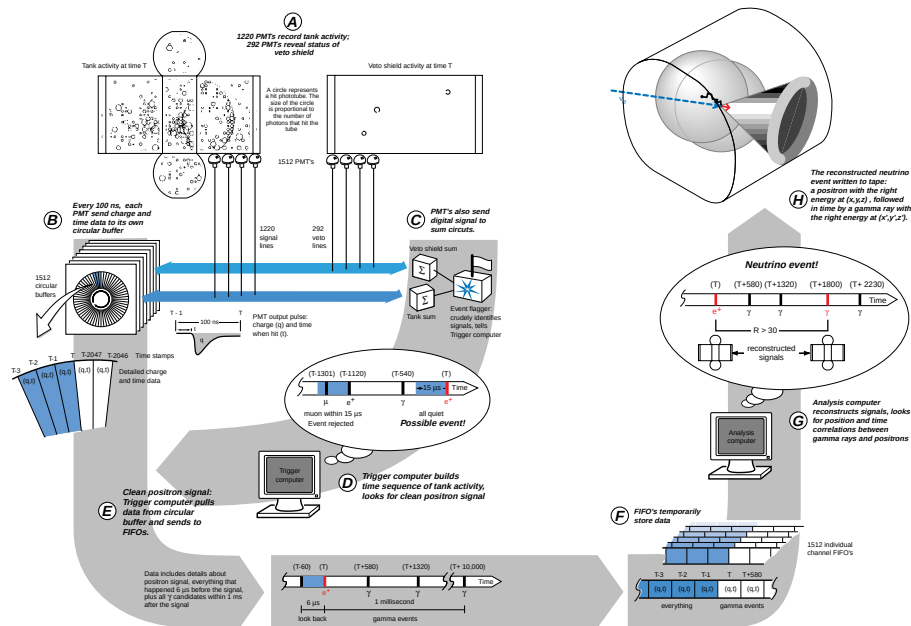
Figure 5.2: The LSND DAQ system.
