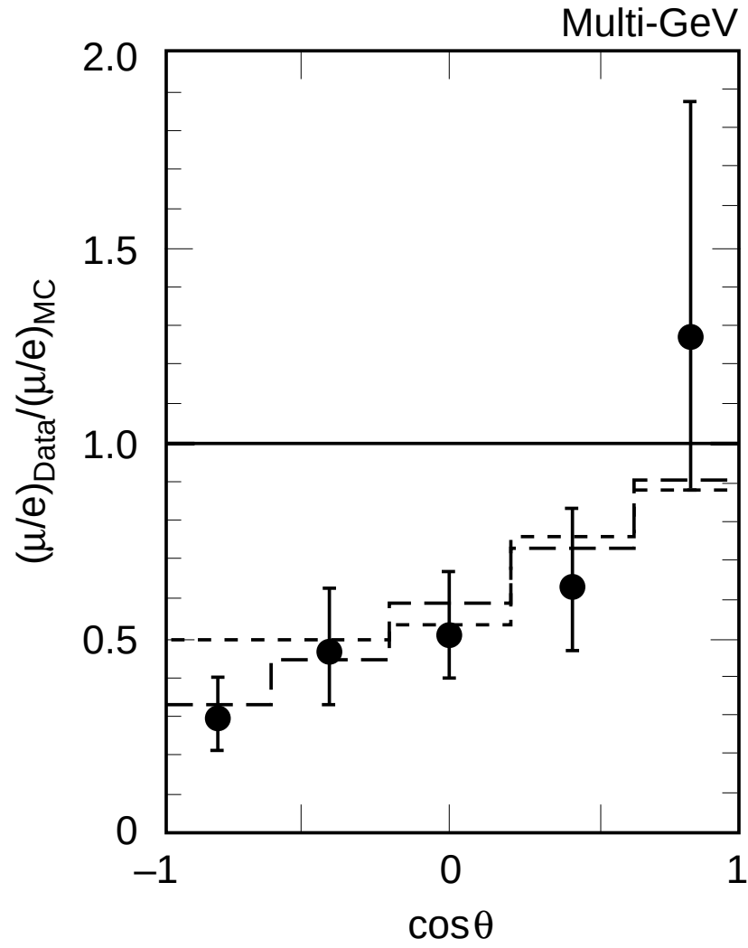
Figure 3.7: Zenith angle distribution of (\mu/e)_{\text{data}}/(\mu/e)_{\text{MC}} from the Kamiokande experiment. The circles with error bars show the data. Also shown are the expectations from the MC simulations with neutrino oscillations for parameter sets (\Delta m^2, \sin^2 2\theta) corresponding to the best-fit values to the multi-GeV data for \nu_\mu \rightarrow \nu_e ( 1.8 \times 10^{-2} \text{ eV}^2, 1.0 ), dashes) and \nu_\mu \rightarrow \nu_\tau ( 1.6 \times 10^{-2} \text{ eV}^2, 1.0 ), dots) oscillations.
