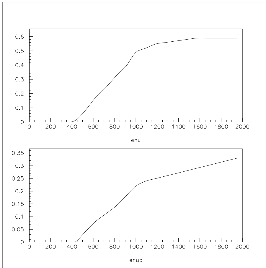
Figure 7.6: The cross sections (in units of 10^{-38} \text{ cm}^2 ) for \nu_\mu C and \bar{\nu}_\mu C neutral current \pi^\pm production as a function of incident neutrino energy in MeV.
