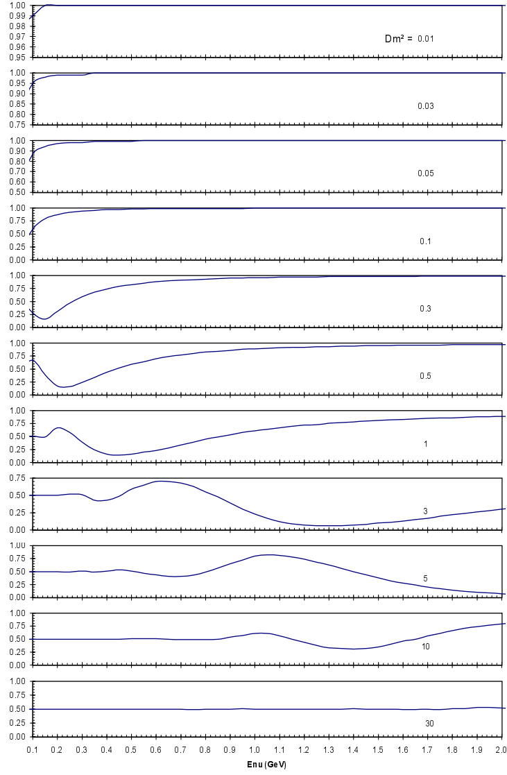
Figure 10.2: The dependence on energy of events at the near (500 m) detector for full mixing and various \Delta m^2 values.
