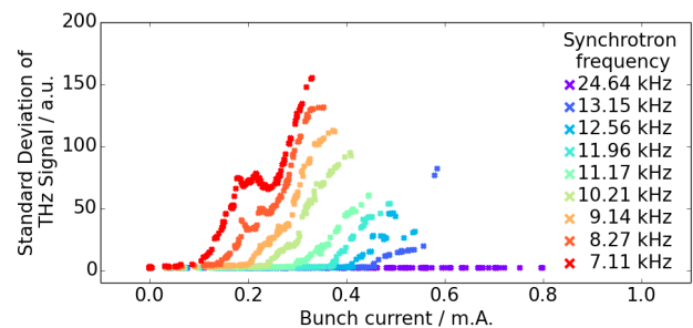
Figure 3: The standard deviation of the THz signal displayed over bunch current is shown for different settings of the magnet optics (with constant RF-voltage), which result in different synchrotron frequencies indicated by color [7].
