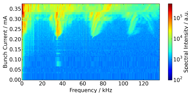
Figure 5: The fast Fourier transform of the THz signal of each bunch is plotted in rows sorted by the bunch current, resulting in a spectrogram showing the development of the bursting frequencies over the current normally obtained by a time consuming decay of one single bunch.
