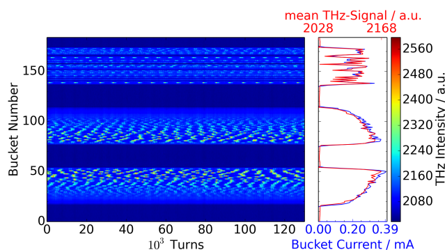
Figure 1: The peak-intensity of the THz pulses of all 184 RF-buckets is displayed over 130 thousand consecutive turns and shows strong fluctuations caused by bursting. A typical measurement takes one second and contains 2.7 million turns. The graph to the right shows the filling pattern.
