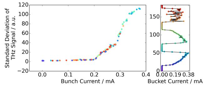
Figure 2: The calculated standard deviation of the THz signal of each bunch is plotted over the corresponding bunch current. The current profile was patterned to resample the whole current range.
