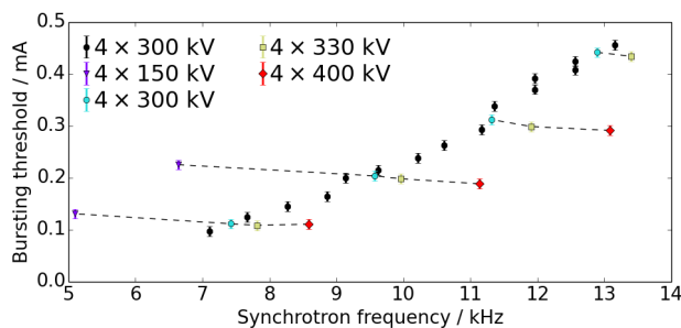
Figure 4: The bursting threshold for a combined scan is shown over the synchrotron frequency. The error bars include the error of the algorithm for the automated threshold detection, the bunch current measurement as well as the expected spread of the threshold due to multi-bunch effects.
