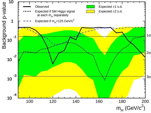
FIG. 8: The significance of the observed data excess with respect to the background-only expectation for the combination of all CDF search channels as a function of SM Higgs boson mass. The probabilities for the background model to result in a best-fit cross section as large or larger than that observed in data, p -values, are shown with the solid line. The dashed line indicates the mean expected p -values in the presence of a SM Higgs boson evaluated separately for each test mass, where the associated shaded regions show the ranges of one and two standard deviation fluctuations in observed p -values for these scenarios. The dot-dashed line indicates mean expected p -values for each mass hypothesis in the case of the SM Higgs boson with m_H = 125 \text{ GeV}/c^2 .
