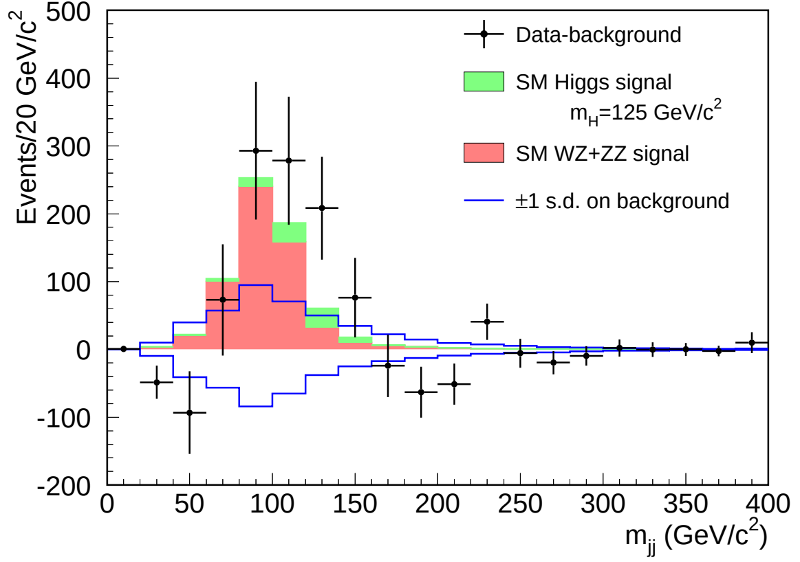
FIG. 2: Background-subtracted dijet invariant mass distribution from the combination of all search channels contributing to the VZ cross section measurement. Expected signal contributions from VZ production (red) and a m_H = 125 \text{ GeV}/c^2 SM Higgs boson (green) are indicated with the filled histograms. The normalization of the subtracted background contribution, with uncertainties indicated by the unfilled histogram, is obtained from a fit to the data.
