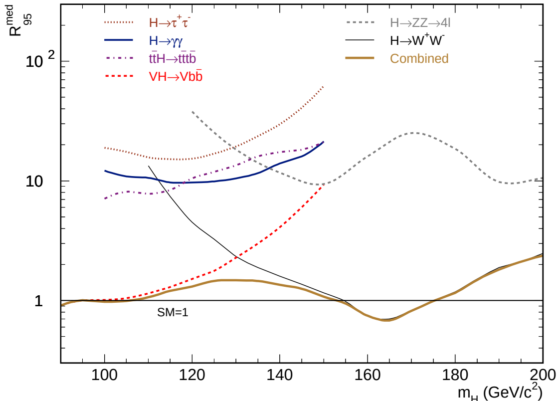
FIG. 2: Median expected 95% C.L. upper limits on Higgs boson production relative to the SM expectation assuming the background-only hypothesis for combinations of search channels within each Higgs boson decay mode and the combination of all search channels as a function of Higgs boson mass in the range between 90 and 200 \text{GeV}/c^2 .
