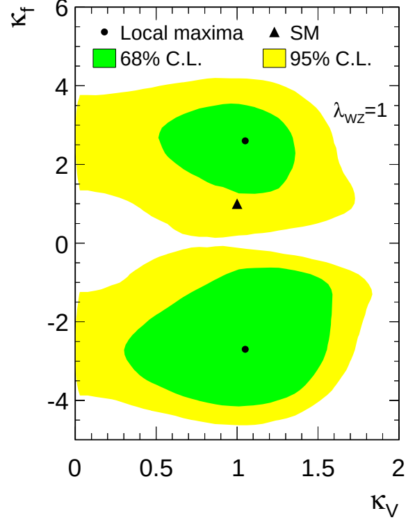
FIG. 17: Two-dimensional constraints in the (\kappa_V, \kappa_f) plane. The 68% and 95% credibility regions are shown. A two-dimensional posterior probability distribution is obtained from a fit to the observed data in all CDF search channels where \kappa_V is the generic Higgs boson coupling to W and Z bosons assuming the SM value of one for \lambda_{WZ} = \kappa_W/\kappa_Z .
