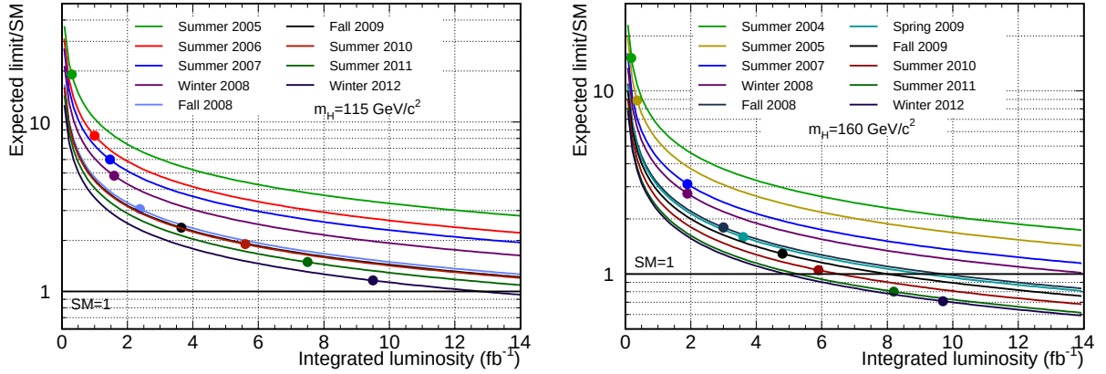
FIG. 3: Achieved and projected median expected 95% C.L. upper limits on Higgs boson production relative to the SM expectation as a function of integrated luminosity, assuming the background-only hypothesis. Each point represents a combination of CDF searches performed on the date indicated in the legend. The integrated luminosity associated with each point is the sensitivity-weighted average of the analyzed luminosities associated with each contributing channel. The solid lines show sensitivity projections, where a scaling inversely proportional to the square root of the integrated luminosity is assumed. The information is provided for combined searches performed at m_H = 115 \text{ GeV}/c^2 (left) and m_H = 160 \text{ GeV}/c^2 (right).
