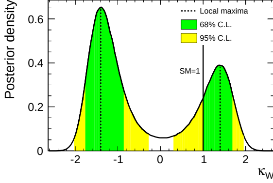
FIG. 13: Posterior probability distribution for \kappa_W from the combination of all CDF search channels. In performing this fit, the values for \kappa_Z and \kappa_f are fixed to their SM values ( \kappa_Z = \kappa_f = 1 ).
