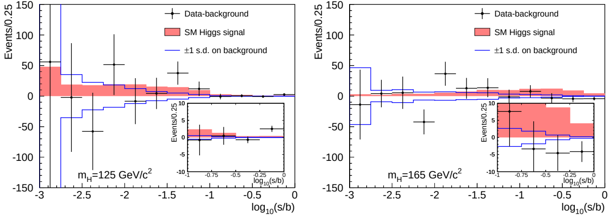
FIG. 5: Background-subtracted collected discriminant histograms, summed for bins with similar signal-to-background ratio ( s/b ), for the combined SM Higgs boson searches focusing on the m_H = 125 \text{ GeV}/c^2 (left) and m_H = 165 \text{ GeV}/c^2 (right) hypotheses. Background normalizations are obtained from fits to the data, and fit uncertainties are indicated by the unfilled histograms. Predicted signal contributions, scaled to SM expectations, are shown with the filled histograms. Uncertainties on the data points correspond to the square root of the sum of expected signal and background yields within each bin.
