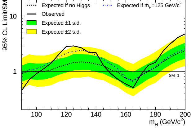
FIG. 6: Observed and expected (median, for the background-only hypothesis) 95% C.L. upper limits on SM Higgs boson production as a function of the Higgs boson mass for the combination of CDF searches. The limits are expressed as multiples of the SM prediction for test masses in 5 \text{ GeV}/c^2 steps from 90 to 200 \text{GeV}/c^2 . The points are connected with straight lines for improved readability. The bands indicate the 68% and 95% probability regions where the limits can fluctuate, in the absence of signal. The lighter dashed line indicates mean expected limits in the presence of a SM Higgs boson with m_H = 125 \text{ GeV}/c^2 .
