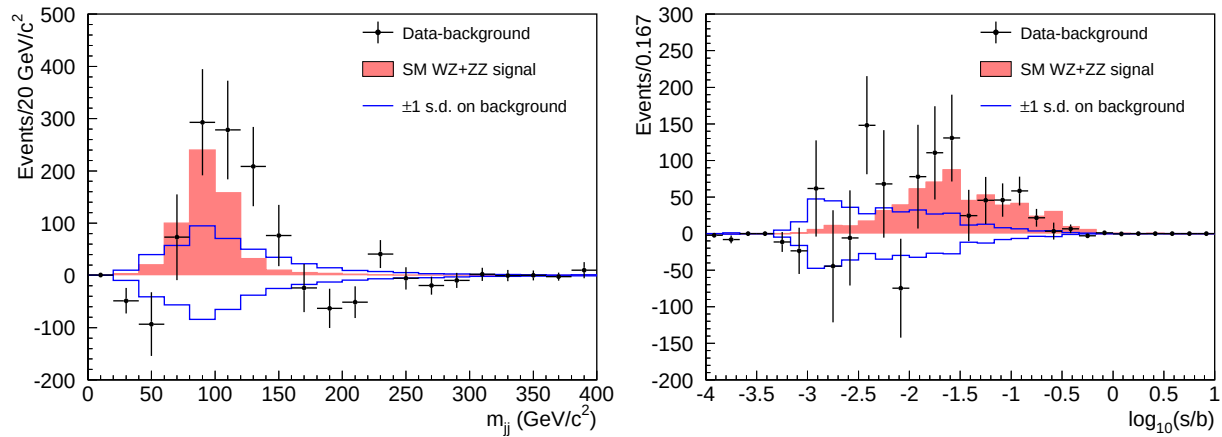
FIG. 1: Background-subtracted dijet invariant mass distribution from the combination of all search channels contributing to the VZ cross section measurement (left) and collected discriminant histograms, summing bins with similar signal-to-background ratio ( s/b ), for the VZ measurement (right). The expected SM signal contributions are indicated with the filled histograms. Normalizations of the subtracted background contributions, with uncertainties indicated by the unfilled histograms, are obtained from fits to the data.
