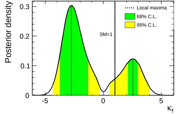
FIG. 15: Posterior probability distribution for \kappa_f from the combination of all CDF search channels. In performing this fit, the values for \kappa_W and \kappa_Z are fixed to their SM values ( \kappa_W = \kappa_Z = 1 ).
