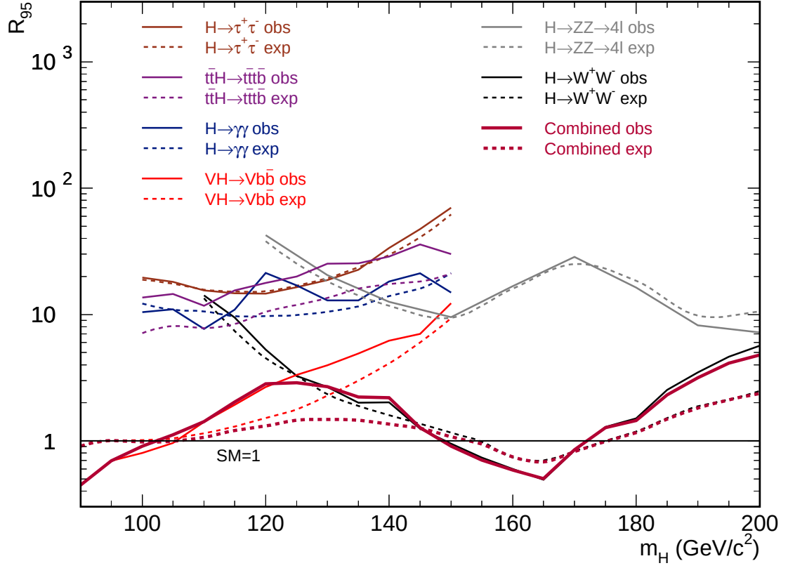
FIG. 1: Median expected (assuming the background-only hypothesis) and observed 95% C.L. upper limits on Higgs boson production relative to the SM expectation for combinations of search channels within each Higgs boson decay mode and the combination of all search channels as a function of Higgs boson mass in the range between 90 and 200 \text{GeV}/c^2 .
