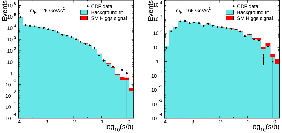
FIG. 4: Collected discriminant histograms, summed for bins with similar signal-to-background ratio ( s/b ), for the combined SM Higgs boson searches focusing on the m_H = 125 \text{ GeV}/c^2 (left) and m_H = 165 \text{ GeV}/c^2 (right) hypotheses. Normalizations of the background contributions are obtained from fits to the data. Predicted signal contributions, scaled to SM expectations, are overlaid on the backgrounds.
