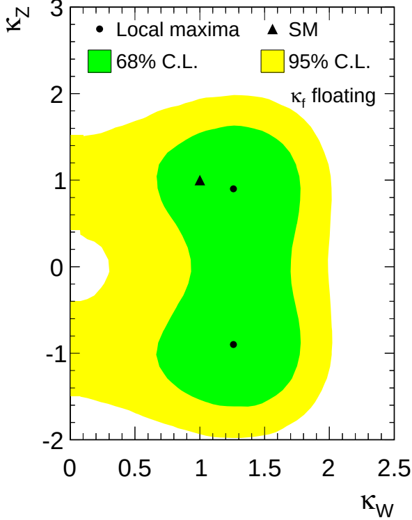
FIG. 16: Two-dimensional constraints in the (\kappa_W, \kappa_Z) plane. The 68% and 95% credibility regions are shown. A three-dimensional posterior probability distribution is obtained from a fit to the observed data in all CDF search channels by floating all three coupling parameters ( \kappa_W , \kappa_Z , and \kappa_f ). The two-dimensional constraints are obtained by integrating the three-dimensional posterior probability density over \kappa_f .
