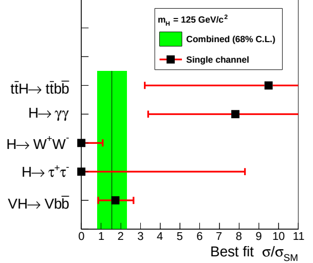
FIG. 9: Summary of best-fit signal cross sections relative to SM expectations for the m_H = 125 \text{ GeV}/c^2 hypothesis. Square dots with horizontal uncertainty bars show the fitted cross sections obtained from the subsets of CDF search channels corresponding to VH \rightarrow Vb\bar{b} , H \rightarrow W^+W^- , H \rightarrow \gamma\gamma , H \rightarrow \tau^+\tau^- , and t\bar{t}H \rightarrow t\bar{t}b\bar{b} production and decay. The solid vertical line and associated shaded region illustrate the fitted SM cross section obtained from all search channels.
