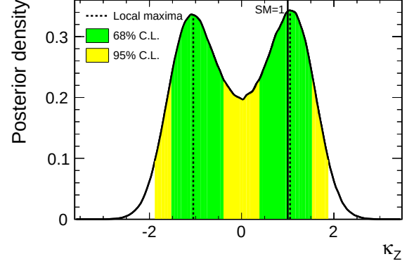
FIG. 14: Posterior probability distribution for \kappa_Z from the combination of all CDF search channels. In performing this fit, the values for \kappa_W and \kappa_f are fixed to their SM values ( \kappa_W = \kappa_f = 1 ).
