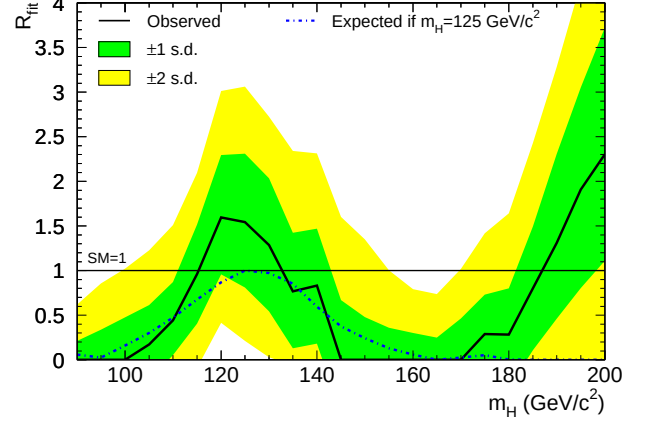
FIG. 7: Best-fit cross section for inclusive Higgs boson production, normalized to the SM expectation, for the combination of all CDF search channels as a function of the Higgs boson mass. The solid line indicates the fitted cross section, and the associated shaded regions show the 68% and 95% credibility intervals, which include both statistical and systematic uncertainties. The mean expected cross section fit values assuming the presence of a SM Higgs boson at m_H = 125 \text{ GeV}/c^2 are shown with the dot-dashed line.
