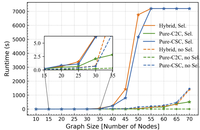
Fig. 3. Runtimes of different networking schemes. The orange curves show the values for hybrid networks; the blue curves denote the values for pure-CSC networks; the green curves denote the values for pure-C2C networks. The solid lines and dotted lines represent the cases with or without untrusted-relay selection respectively.
