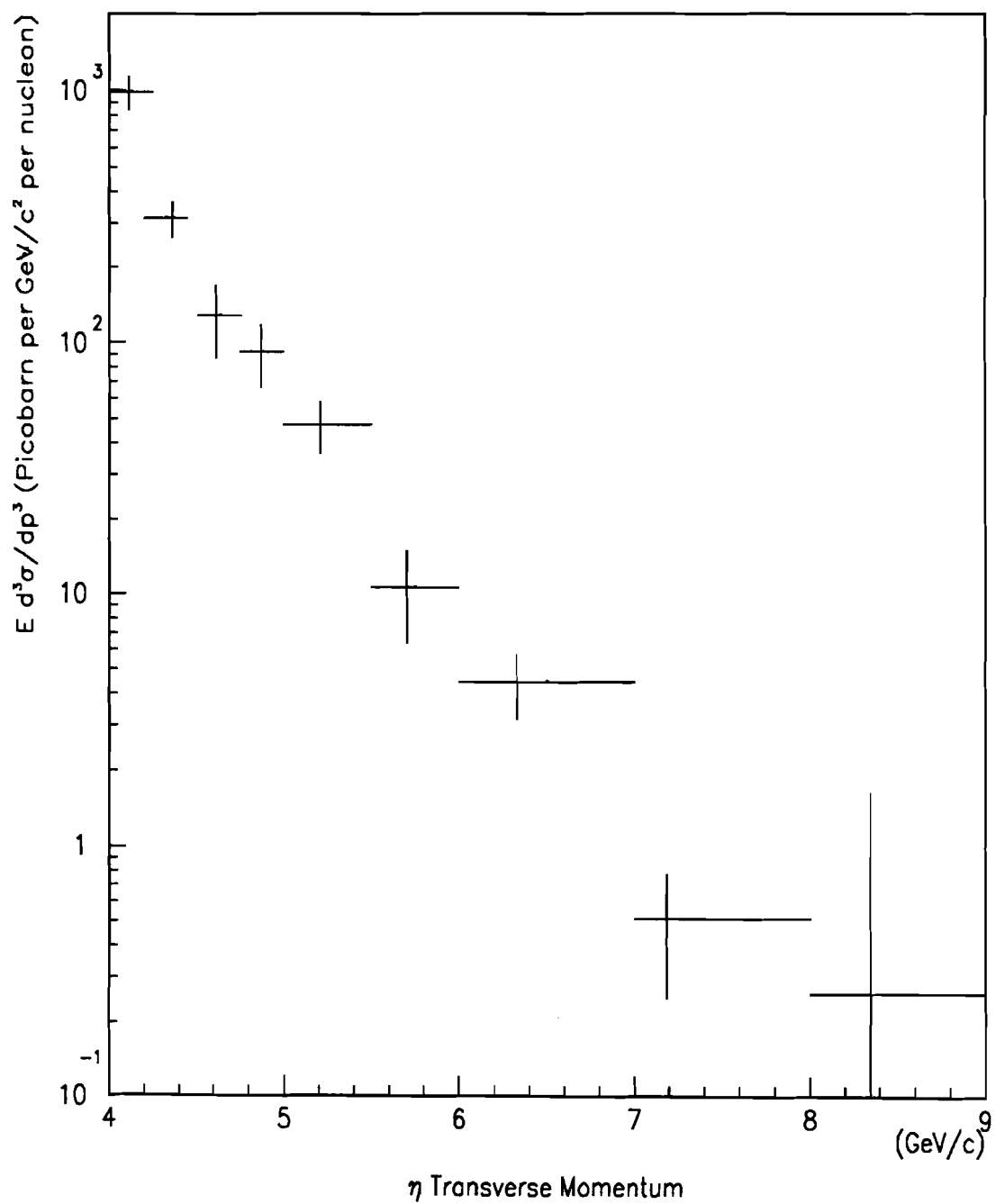
Figure 52: E \frac{d^3\sigma}{dp^3}(\pi^- + Be \rightarrow \eta + X) as a function of P_T for P_T greater than 4. \text{GeV}/c .
