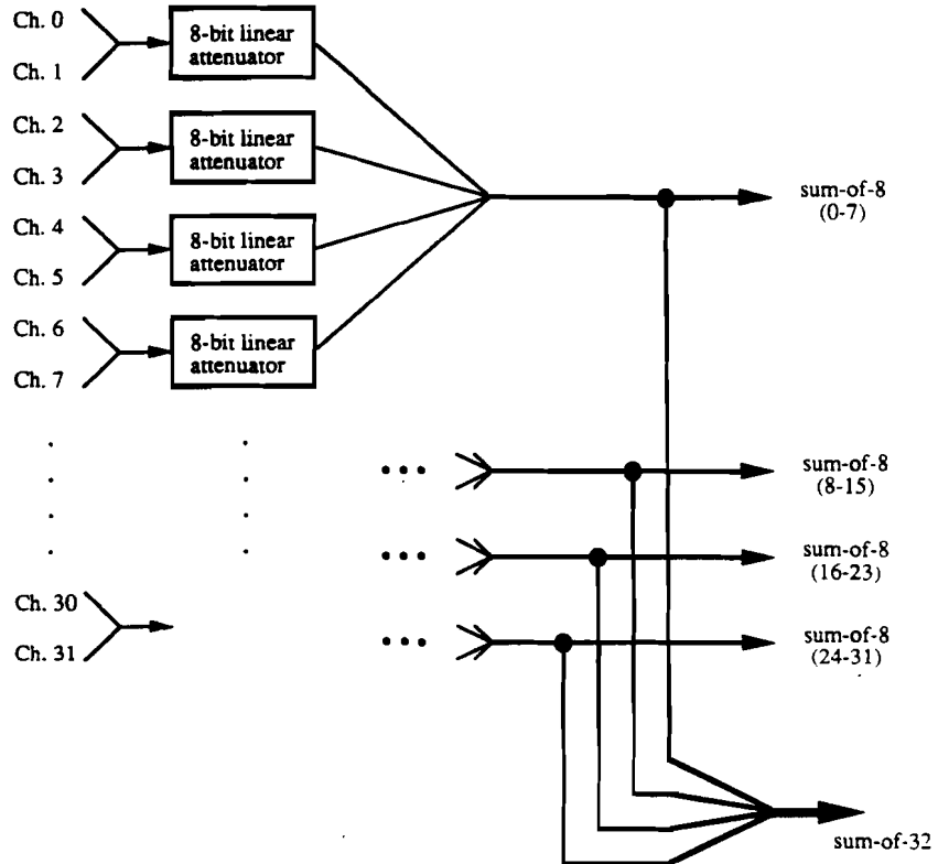
Figure 33: The E706 P_T Summing Module.
