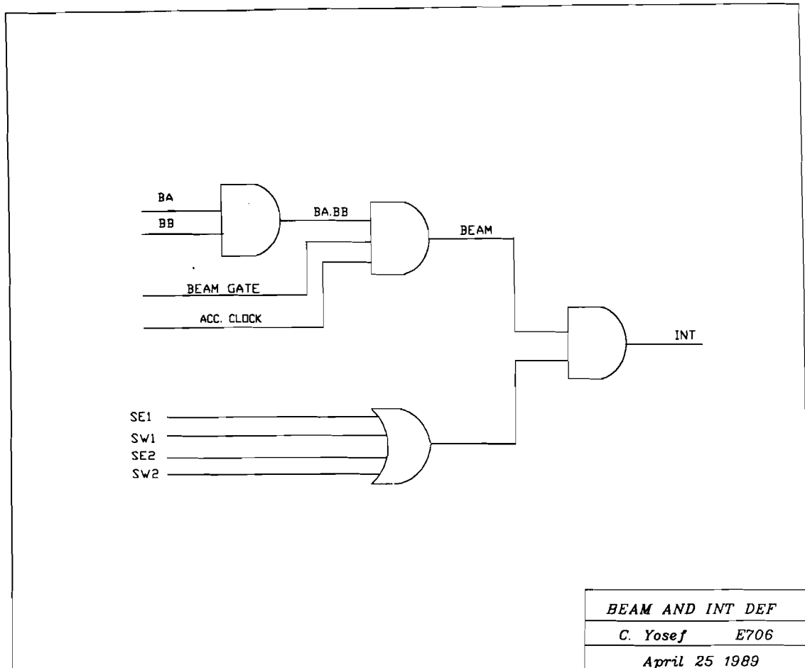
Figure 30: Trigger Logic showing INT and LIVE_INT1.
