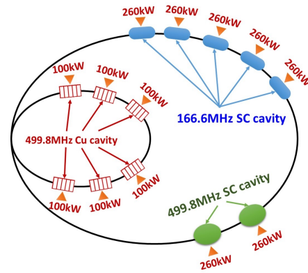
Figure 1: Layout of the HEPS RF system.
