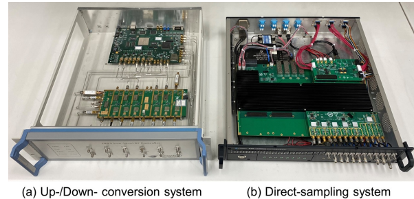
Figure 7: 166.6 MHz LLRF system prototype.
