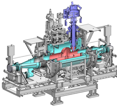
Figure 4: 499.8 MHz SRF cavity module.
