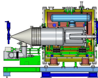
Figure 3: 166.6 MHz SRF cavity module.
