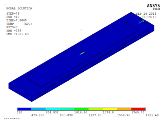
Figure 7: The temperature distribution on beam impacting surface.
