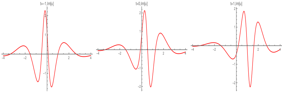
Fig. 2. \text{Im}[u] in (85) with the parameters chosen as \xi_1 = 1 , \eta_1 = 1 , \alpha_0 = \beta_0 = 0 .
