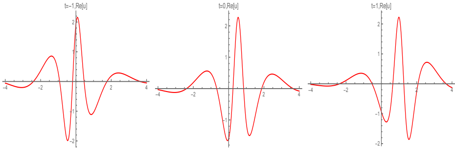
Fig. 1. \text{Re}[u] in (85) with the parameters chosen as \xi_1 = 1 , \eta_1 = 1 , \alpha_0 = \beta_0 = 0 .
