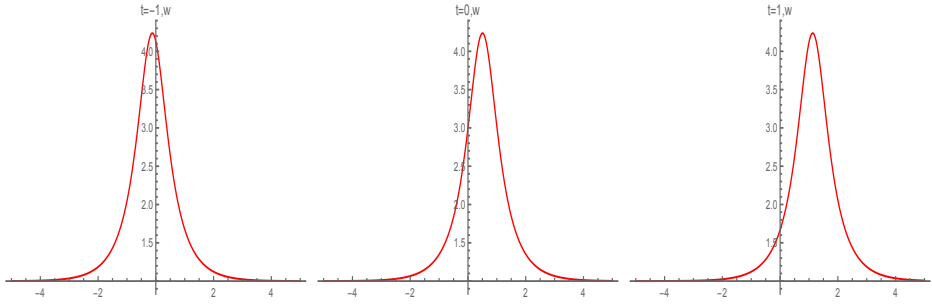
Fig. 4. w(x, t) in (85) with the parameters chosen as \xi_1 = 1, \eta_1 = 1, \alpha_0 = \beta_0 = 0 .
