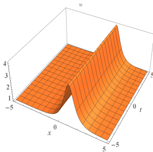
Fig. 6. w(x, t) in (85) with the parameters chosen as \xi_1 = 1, \eta_1 = 1, \alpha_0 = \beta_0 = 0 .
