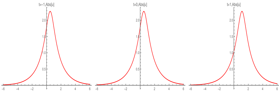
Fig. 3. \text{Abs}[u] in (85) with the parameters chosen as \xi_1 = 1 , \eta_1 = 1 , \alpha_0 = \beta_0 = 0 .
