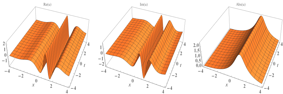
Fig. 5. \text{Re}[u], \text{Im}[u], \text{Abs}[u] in (85) with the parameters chosen as \xi_1 = 1, \eta_1 = 1, \alpha_0 = \beta_0 = 0 .
