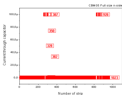
Figure 6: Pinhole test of the CBM05 sensor prototype.
