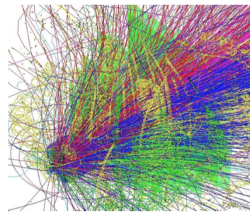
Figure 2: A simulated Au-Au collision at 25 AGeV energy with about 1000 charged particles produced.
