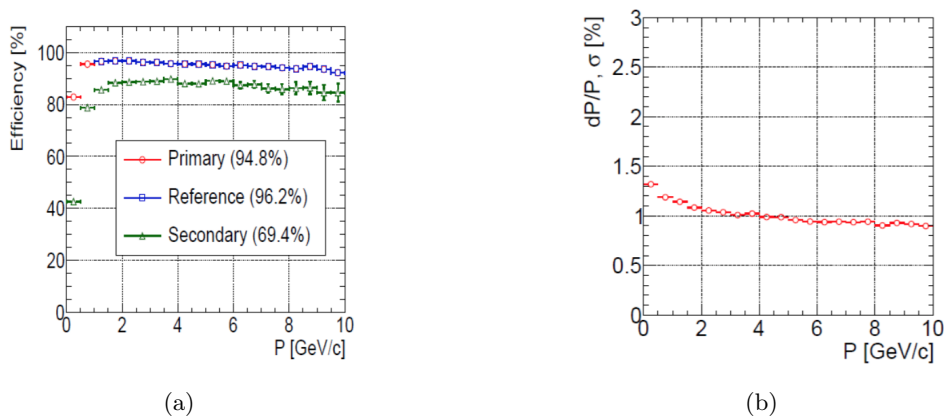
Figure 5: Track reconstruction efficiency (a) and momentum resolution (b) in the STS as a function of momentum for all tracks in central Au-Au collision at 25 AGeV.
