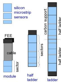
Figure 3: STS building blocks.
