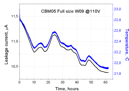
Figure 9: Leakage current and temperature monitoring.
