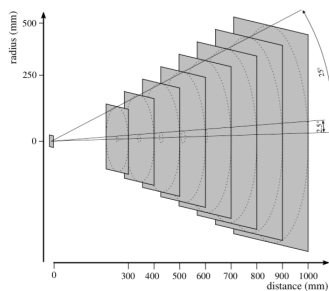
Figure 1: STS stations concept.
