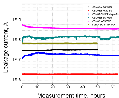
Figure 8: Long-term stability test of the CBM sensor prototypes.
