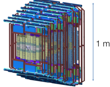
Figure 4: View of the assembled tracking stations.
