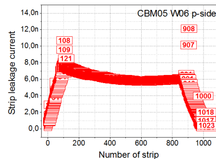
Figure 7: Measurement of the strip leakage current distribution of the CBM05 sensor prototype.
