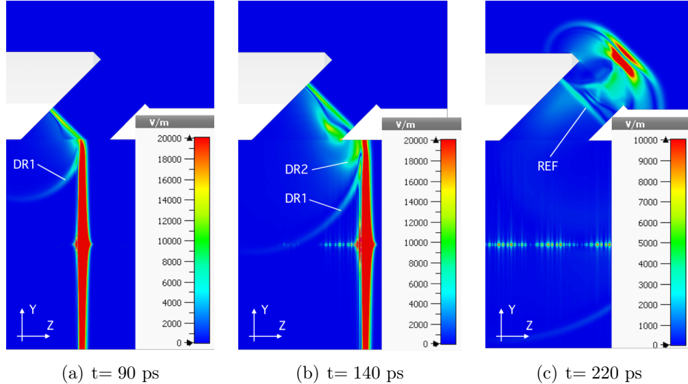
Figure 3.10: 3D simulation of the electric field produced by the beam passing next to a PTFE radiator with the same geometry as the one used for the tests at CLEAR. The grey and white areas represent the metal pipe. The ChDR and DR front formations are visible and are described in detail in the text.
