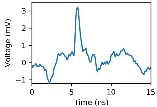
(b) Output signal
