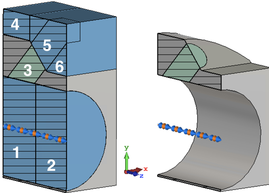
Figure 3.9: Longitudinal section of the 3D model used for the electromagnetic simulations. On the left the model is displayed including the vacuum parts and indicating the different meshing regions, on the right the vacuum volumes are hidden. Light blue volumes are made of vacuum, light green volume is the PTFE radiator, and volumes in grey are metal. The orange and blue arrows indicate the propagation path and direction of the beam.
