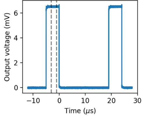
Figure 3.17: An RF diode installed on the synthesizer for calibration (left) and a typical diode output signal during calibration (right). Only the region between the dashed lines is taken into account to evaluate the average voltage output. The rise and fall of the pulse are discarded, as it is not possible to assess to which extent these are determined by the diode or the synthesizer. Additional details on the response of Schottky diodes to fast transients are given in Section 3.4.5.
