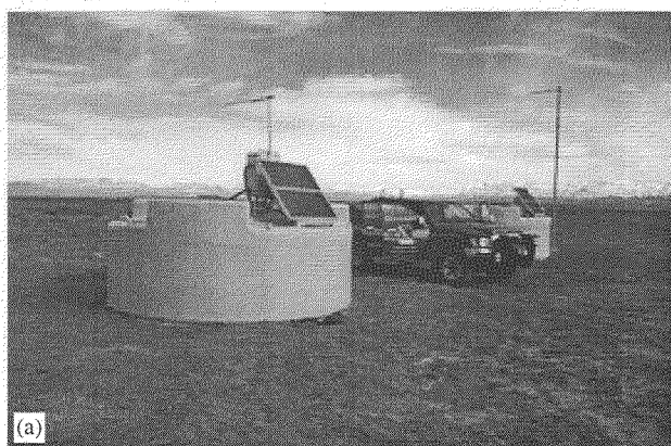
Fig. 4. (a) The Carmen and Miranda tank pair; (b) timing difference for low-energy showers triggering the Carmen-Miranda pair. The 17 ns sigma Gaussian distribution corresponds to an individual resolution of 8 ns for each tank. The 50 ns offset is a stable offset that is characteristic of this receiver pair.
