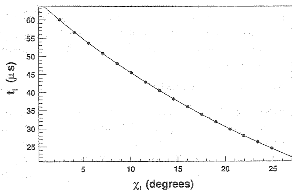
Fig. 27. An example of the geometry associated with shower reconstruction. The measured pixel time t_i is plotted as a function of \chi_i , the direction of pixel i projected onto the SDP. The closed dots are experimental data, the solid line is the result of the fit.
