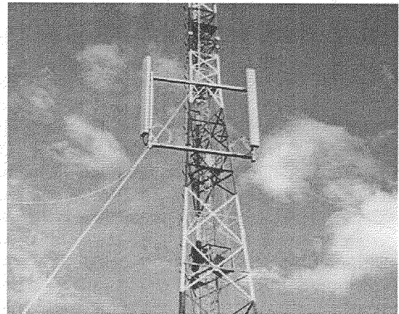
Fig. 17. Base station panel antennas being installed at Los Leones.
