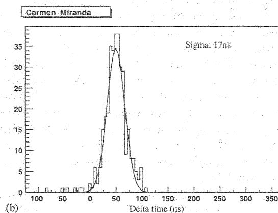
Fig. 4. (a) The Carmen and Miranda tank pair; (b) timing difference for low-energy showers triggering the Carmen-Miranda pair. The 17 ns sigma Gaussian distribution corresponds to an individual resolution of 8 ns for each tank. The 50 ns offset is a stable offset that is characteristic of this receiver pair.
