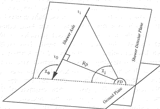
Fig. 26. SDP and shower geometry.
