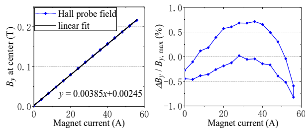
Figure 7: Magnet excitation and linear fit (left), and field deviation from linearity (right) of the first dipole.
