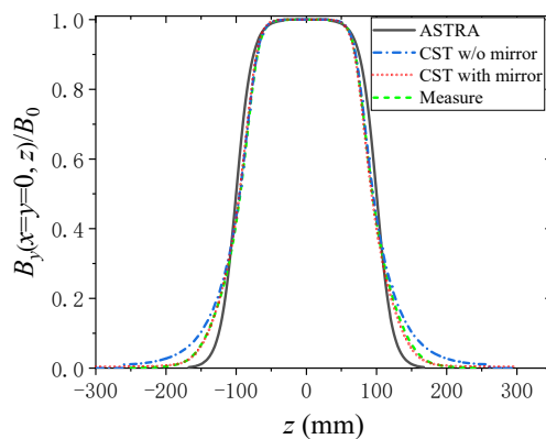
Figure 4: Normalized vertical field component along axis.
