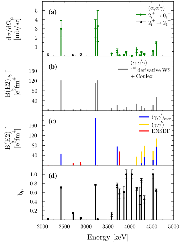
Fig. 4. (Color online.) (a) \alpha -scattering cross sections. States decaying to the ground state are shown in green. States, which have not been observed to decay to the ground state but to the 2_1^+ state are shown in black. (b) B(E2)_{\text{IS}}\uparrow values deduced from the \alpha -scattering cross sections, see text. (c) B(E2)\uparrow values from NRF measurements in blue. Values below 4 MeV are adopted from Ref. [54]. The feeding-corrected values above 4 MeV have been determined in this work. For completeness, the uncorrected values are also presented in yellow. In red, additionally adopted values from Ref. [53] are shown. (d) Ground-state \gamma -decay branching ratio b_0 = \Gamma_0/\Gamma .
