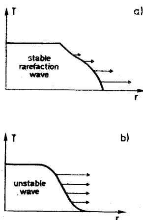
Fig. 5. (a) Temperature profile in a simple one dimensional rarefaction wave. The arrows indicate schematically the velocity of the flow pattern. (b) Same as 5a but for a speed of sound which violates the condition (4.4)
