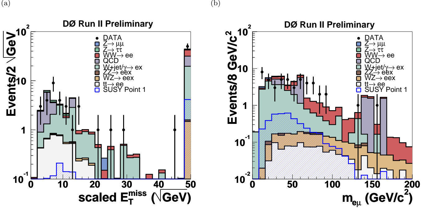
FIG. 2: (a) Distributions in the scaled missing transverse energy (a) after the minimal transverse mass criterion (Cut 1) and (b) the invariant mass for Monte Carlo and data after the E_T selection (Cut 2). The last bin in distribution (a) reflects all the events without any good reconstructed jet.
