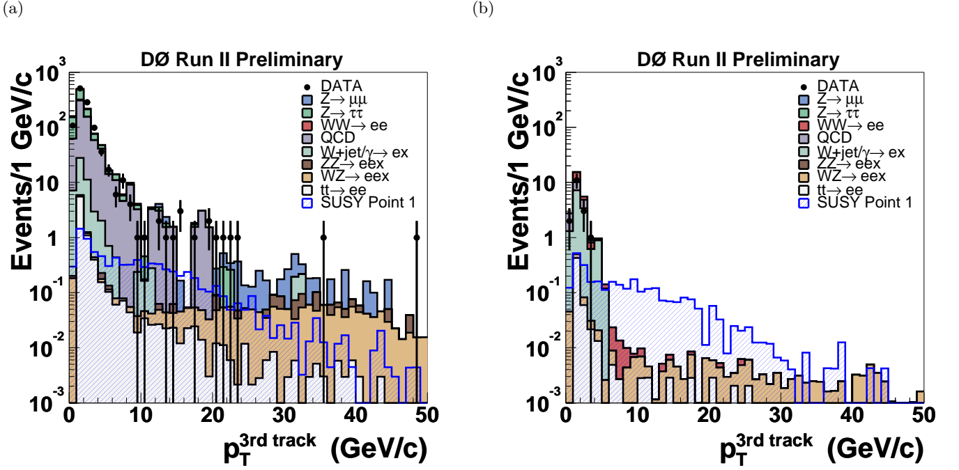
FIG. 3: Distributions in p_T of the third isolated track for the initially selected 1305 events (a, Cut 0) and (b) before the p_T requirement on the third track is imposed (Cut 5).
