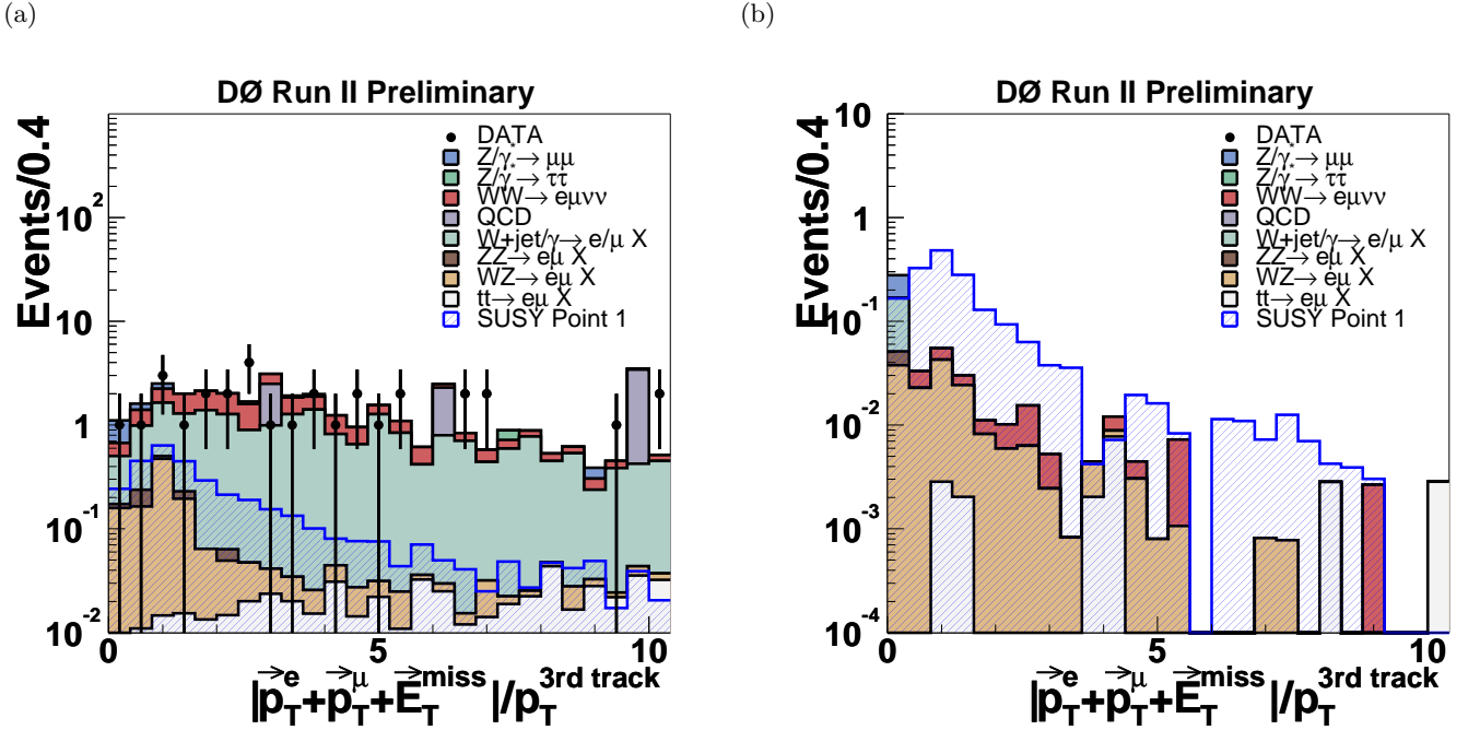
FIG. 4: Distributions in |\vec{p}_T^e + \vec{p}_T^\mu + \vec{E}_T^{\text{miss}}|/p_T^{\text{3rd track}} after applying Cut 2 (a) and (b) before applying Cut 7.
