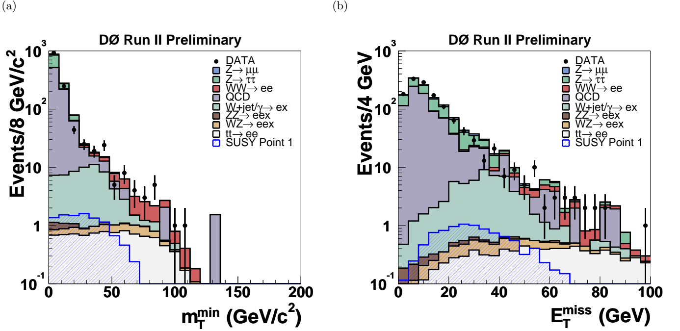
FIG. 1: (a) Distribution in the smaller of the transverse masses and (b) the missing transverse energy after lepton identification and kinematic criteria.
