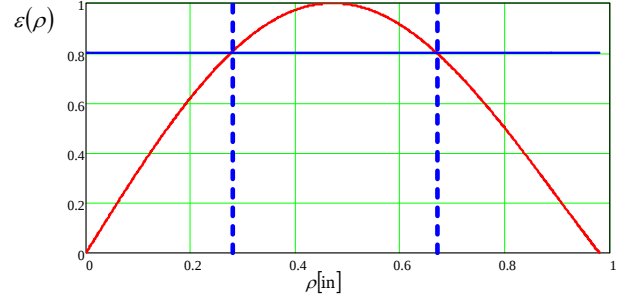
Figure 5: Normalized surface magnetic field.
