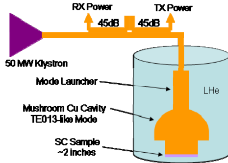
Figure 1: Simplified schematic showing a klystron, a mode launcher, a mushroom cavity and transmitted and reflected pickup ports.
