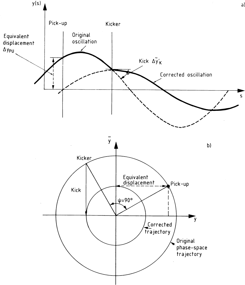
Fig. 13 Real-space diagram (a) and phase-space diagram (b) of betatron oscillation between pick-up and kicker. In smooth approximation the change \Delta \tilde{y}' of normalized angle [y'(R/Q)] is equivalent to a change of position \Delta y_{pu} = \Delta \tilde{y}' at the pick-up at a phase \Delta \psi = Q(\Delta s/R) = 90^\circ (+ k \cdot 180^\circ) upstream.
