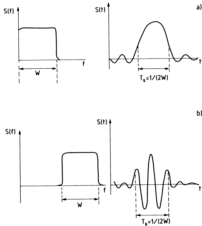
Fig. 4 Illustration of the Küpfmüller-Nyquist relation: A signal whose Fourier decomposition S(f) has a bandwidth W has a typical time duration T_s = 1/(2W) . Illustration for a 'low pass' [case (a)] and a 'band-pass' signal [case (b)].
