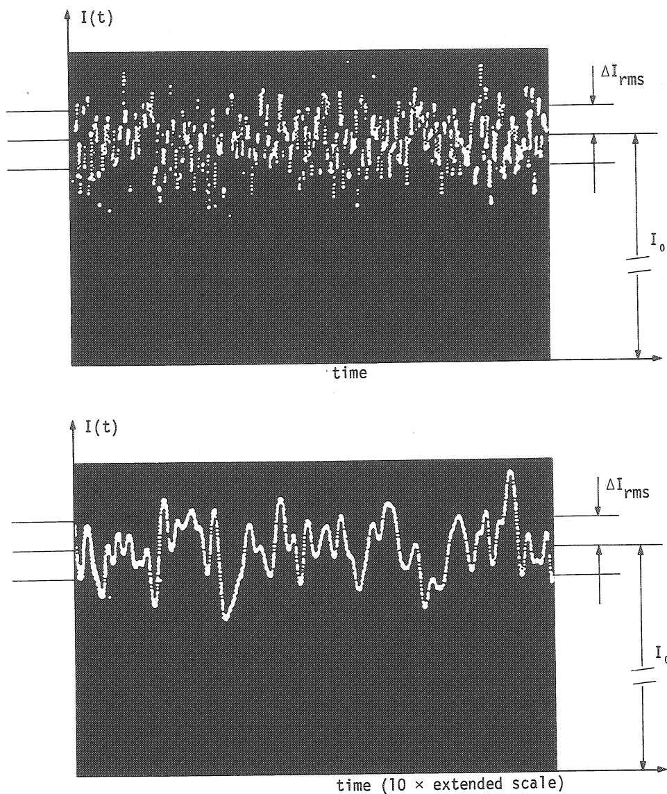
Fig. 4 The pick up current I(t) of a coasting beam consists of a DC current I_0 \propto N and a fluctuating (noise) component with an r.m.s. \sqrt{\Delta(I)^2} = \Delta I_{rms} \propto \sqrt{N} . The highest frequencies resolved are given by the bandwidth of the acquisition system.
