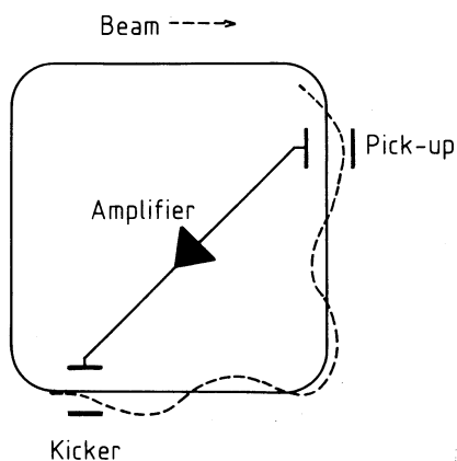
Fig. 1 The principle of (horizontal) stochastic cooling. The pick-up measures horizontal deviation; the kicker corrects angular error. They are spaced by a quarter of the betatron wavelength \lambda_\beta (plus multiples of \lambda_\beta/2 ). A position error at the pick-up transforms into an error of angle at the kicker. This error of angle is corrected.
