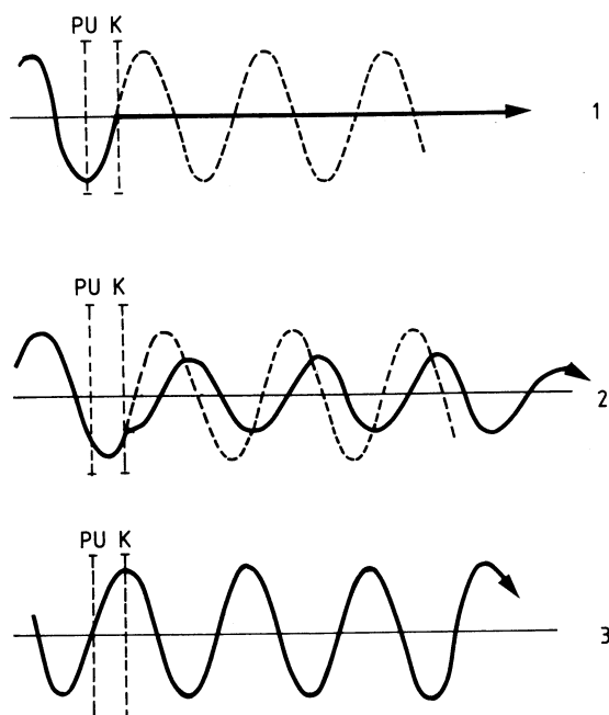
Fig. 2 The importance of betatron phase: Particle 1 crosses the pick-up with maximum elongation. Its oscillation is (ideally) completely cancelled at the kicker. Particle 2 arrives at an intermediate phase; its oscillation is only partly eliminated. Particle 3 arrives with the most unfavourable phase and is not affected by the system.
