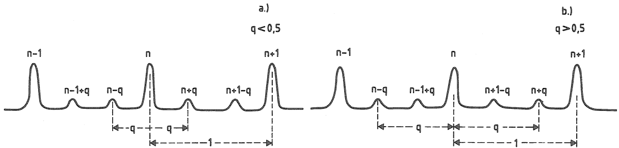
Fig. 10 Position of sidebands (n \pm Q)f_0 where q is the non-integer part of the betatron tune Q . For q < 0.5 the two bands right and left of a revolution harmonic n are the bands (n \pm q)f_0 (fig. 10a). For q > 0.5 the two bands closest to n are the n + 1 - q and n - 1 + q bands (fig. 10b).
