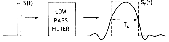
Fig. 5 Input and output signal S(t) of a band-pass system and 'rectangular' approximation to the output pulse S_f(t) .
