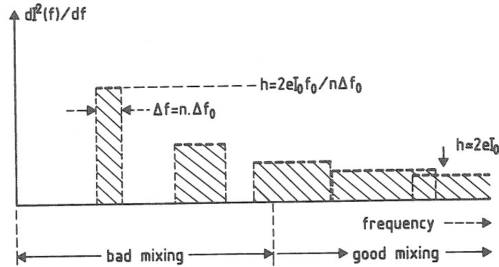
Fig. 6 Schottky noise bands (rectangular approximation) of a coasting beam. The n^{\text{th}} band, centred at nf_0 , has a width n\Delta f_0 and an effective height 2Ne^2 f_0 \cdot f_0 / n\Delta f_0 . The bands describe the power spectrum of the current fig. 4; f_0 \pm \Delta f_0/2 is the range of revolution frequencies. At high harmonics ( n > f_0/\Delta f_0 ) bands overlap and the height (spectral density) of the noise power is 2Ne^2 f_0 = 2eI_0 as for classical shot noise. The width of the bands is exaggerated.
