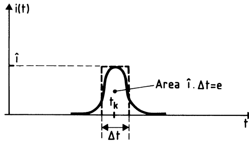
Fig. 1 The current pulse due to a single particle passing a longitudinal pick up and its equivalent square pulse. The area under the pulse \int i(t) dt = \hat{i} \cdot \Delta t = e is given by the charge which has passed the pick up. The transit time \Delta t depends on the length and the shape of the electrodes as well as on the particle velocity. Except for very high frequency, i(t) can be approximated by a \delta -function e\delta(t-t_k) .
