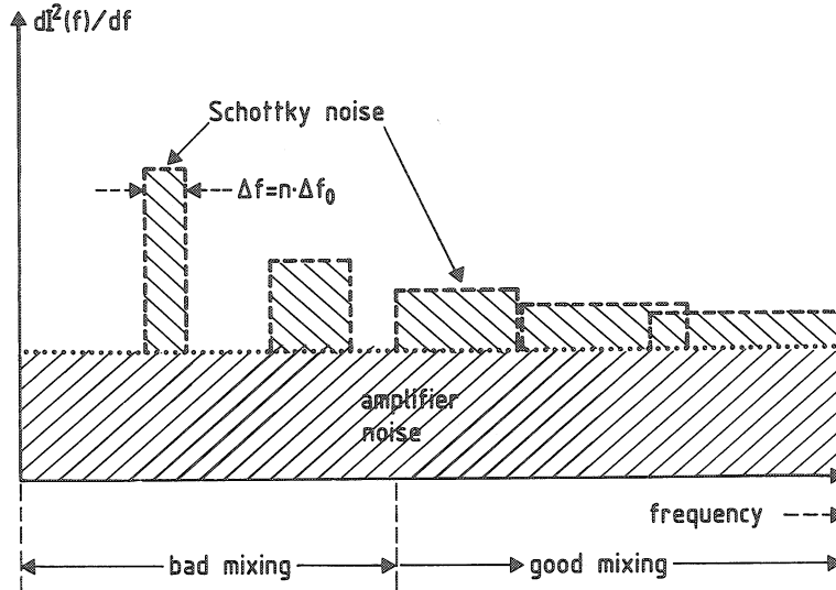
Fig. 7 Amplifier and Schottky noise which determine the incoherent heating. The amplifier noise has a continuous spectrum with a density dI^2/df = 10^{\nu/10} k T_e/R given by the noise figure \nu of the low level system. The Schottky noise has the band spectrum, fig. 6. The width of the bands is exaggerated.
