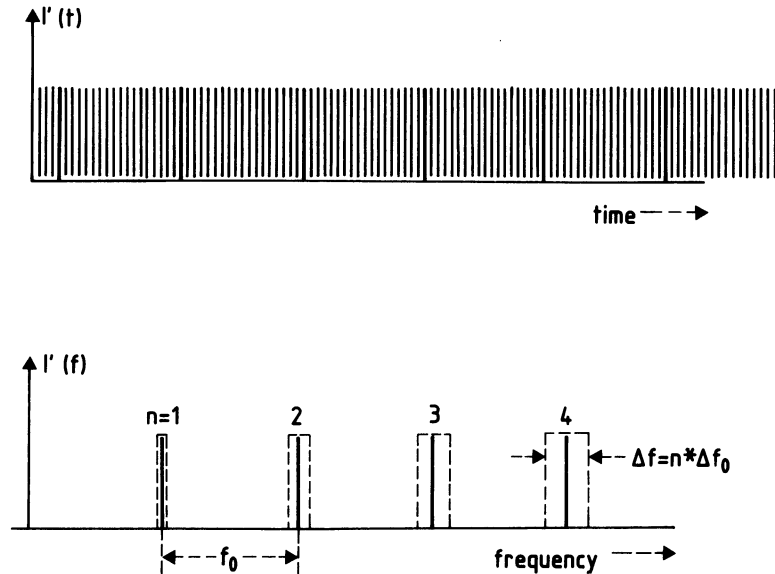
Fig. 3 Time and frequency spectrum of a group of particles with a distribution of revolution frequencies f_0 \pm \Delta f_0/2 . The n th band of the frequency spectrum has a width n\Delta f_0 . The height of the bands is arbitrary at this stage.
