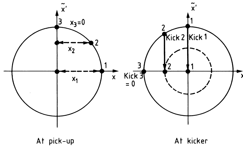
Fig. 3 Phase space representation of betatron cooling. The same as for Fig. 2 except that a 'polar diagram' R/Q \ x' = f(x) is used to represent the betatron motion x = \hat{x} \sin [Q(s/R) + \psi_0] , (R/Q) \ x' = \hat{x} \cos [Q(s/R) + \psi_0] . The undisturbed motion of a particle is given by a circle with the radius equal to the betatron amplitude \hat{x} . Kicks correspond to a jump of x' . The cooling system tries to put particles onto smaller circles. Particles 1, 2, and 3 are sketched with the most favourable, the intermediate, and the least favourable initial phase, respectively. As the number of oscillations per turn is different from an integer or half-integer, particles come back with different phases on subsequent turns and all particles will be cooled progressively.
