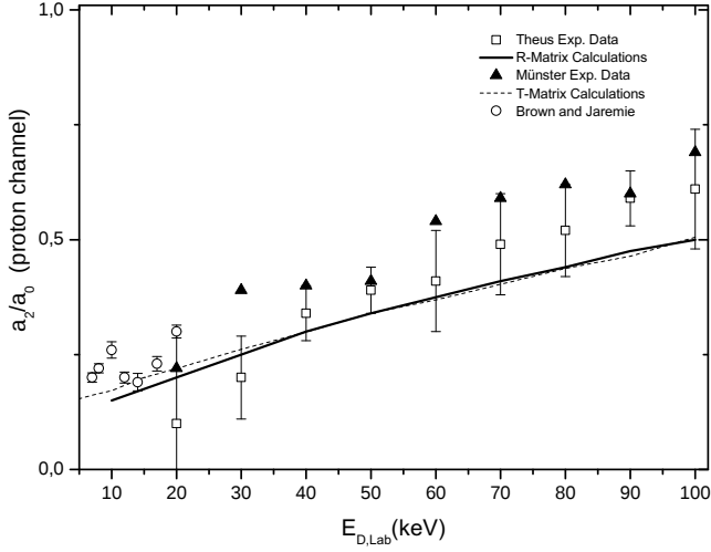
Fig. 1. T-matrix and R-matrix [12] calculations of the anisotropy coefficient for the ^2\text{H}(d,p)^3\text{H} reaction compared to the experimental data of Theus [14], Münster [15], Brown and Jarmie [16].
