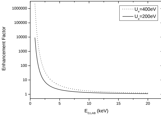
Fig. 4. Enhancement factor for screening energies of 200 eV and 400 eV.
