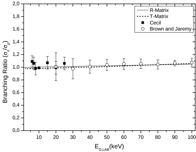
Fig. 2. Experimental and theoretical neutron-to-proton branching ratio. The experimental data are from Ref. [17] and [16].
