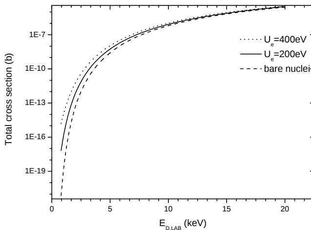
Fig. 3. Total cross section for the {}^2\text{H}(d,p){}^3\text{H} reaction including the screening energies of 200 eV and 400 eV.
