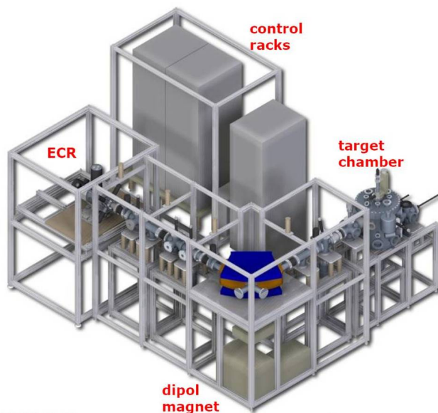
Fig. 5. New accelerator facility with UHV at the University of Szczecin.
