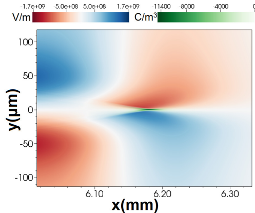
Figure 3: Overlay of the bunch charge density on to the transverse electric field after 6 mm propagation for the short pulse mode.
