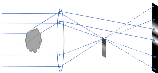
Figure 2: Formation of schlieren image of gas flow.
