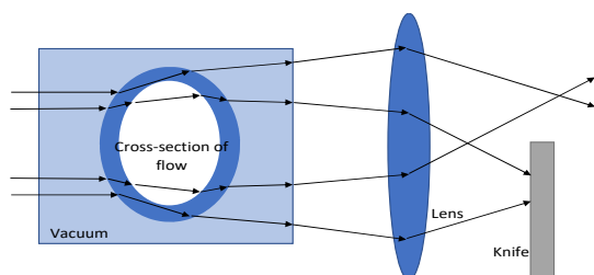
Figure 6: Deflection of light in the schlieren setup by the cross section of the flow.
