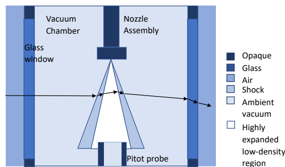
Figure 5: The deflection of a single light ray (Top view).
