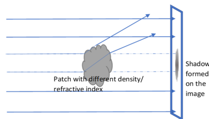
Figure 1: Formation of shadow image of gas flow.
