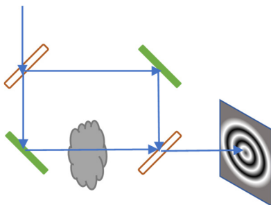
Figure 3: Formation of interference image of gas flow.
