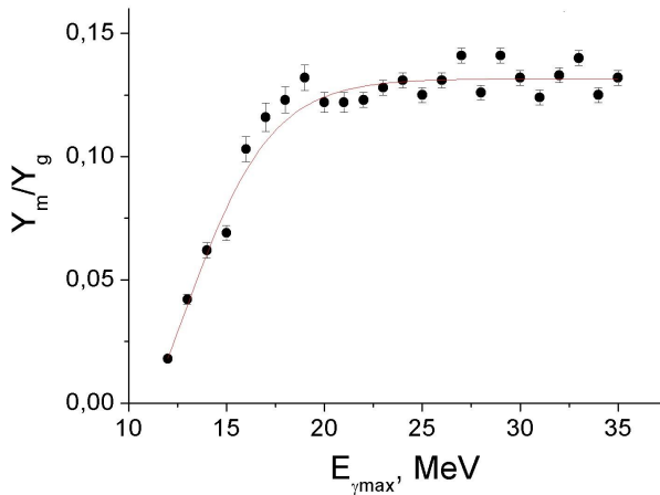
Fig.1. Energy dependences of isomeric ratios of the yields of the reaction ^{140}\text{Ce}(\gamma, n)^{139m,g}\text{Ce} .
